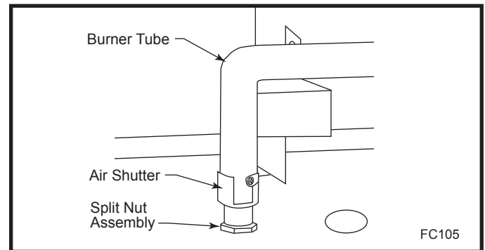
Fig. 46 Loosen split nut assembly from air shutter and remove burner tube.
