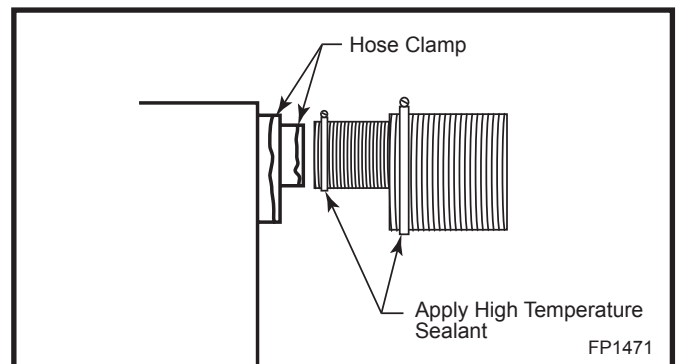
Fig. 8 Apply high temperature sealant to 4" and 7" pipes.
