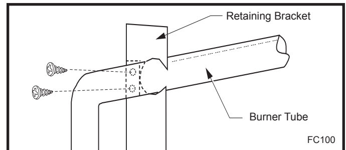
Fig. 45 Bend retaining bracket away from tube.
