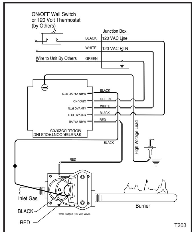
Fig. 44 Electronic ignition module wiring diagram.
