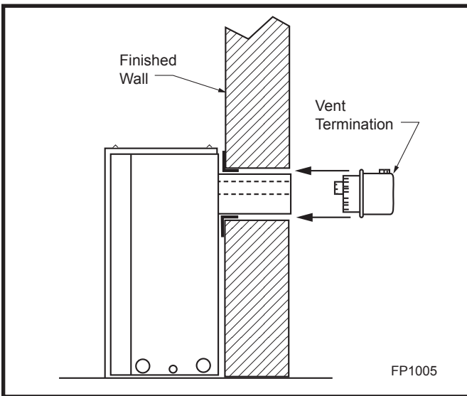
Fig. 15 Side view of final unit location.
