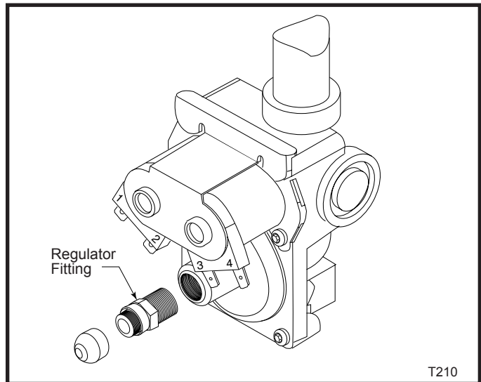
Fig. 50 White-Rodgers 25M18A-706PI gas control.
