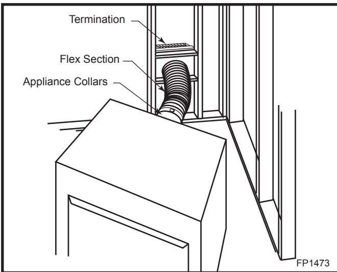
Fig. 16 Grasp the vent pipe close to the collar and bend to 45° angle. Do not exceed 45°.
