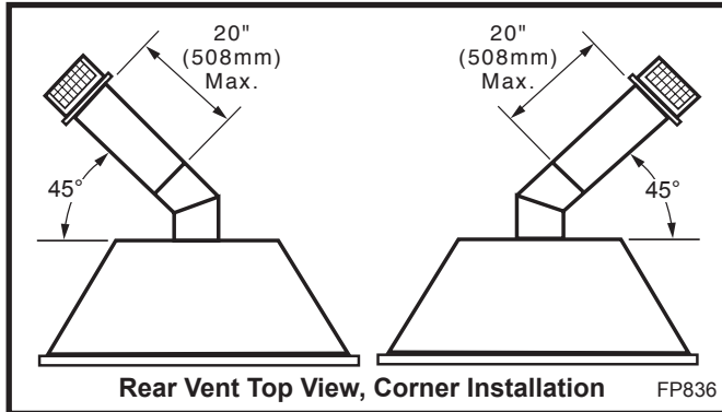
Fig. 12 Rear vent application, one 45° elbow.
