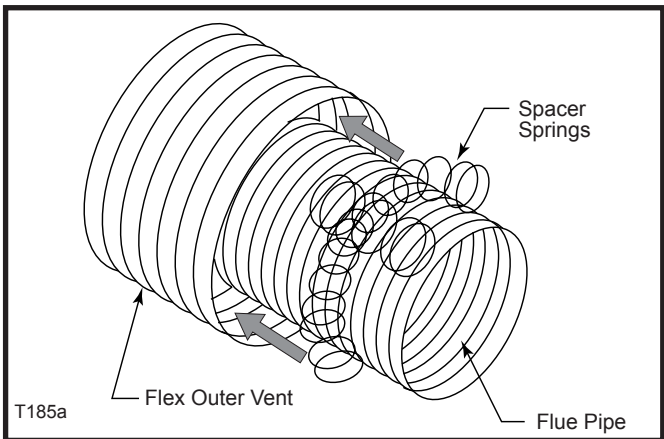
Fig. 28 Wrap spacer spring around flex flue pipe, overlapping ends.
