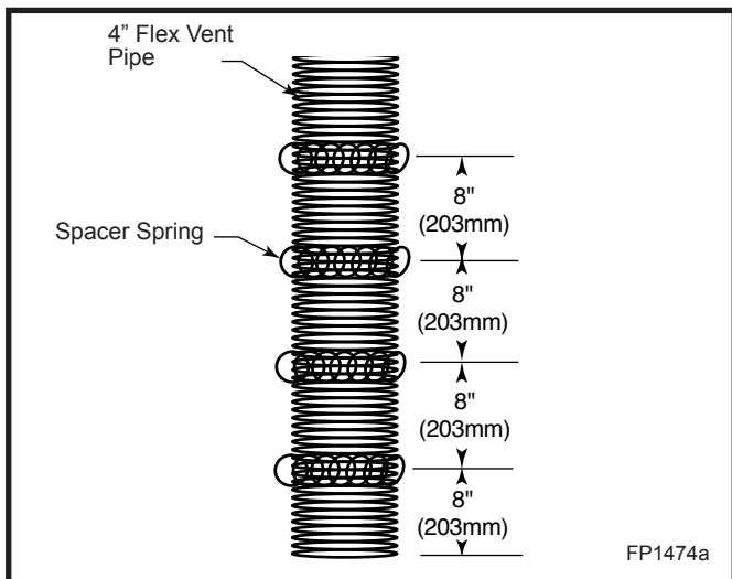
Fig. 29 Install spacer springs.
