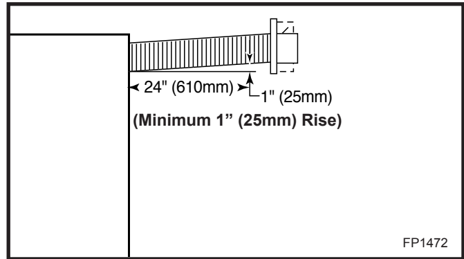
Fig. 17 There must be a 1" rise in 24" length.
