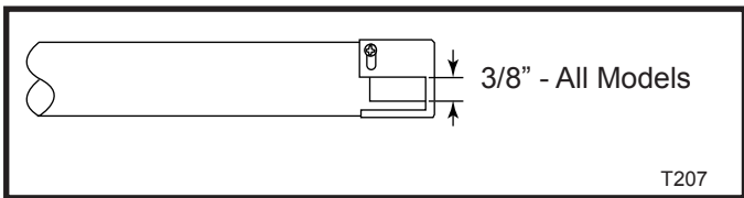
Fig. 49 Air shutter settings for propane/LP gas.
