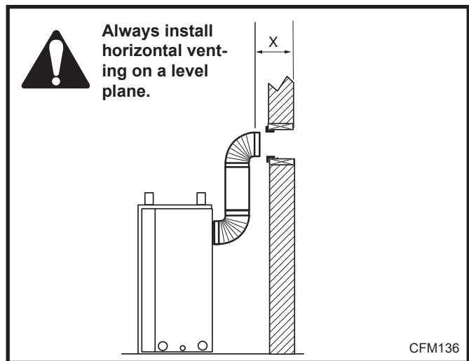
Fig. 25 Measure horizontal length including 2" overlap.
