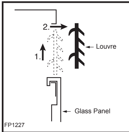
Fig. 38 Remove top louvre assembly.
