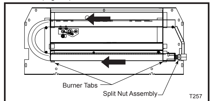
Fig. 47 Bend tabs down, loosen split nut assembly and slide burner tube to the left.
