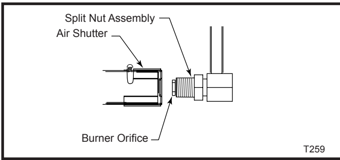
Fig. 48 Replace burner orifice with correct conversion orifice.
