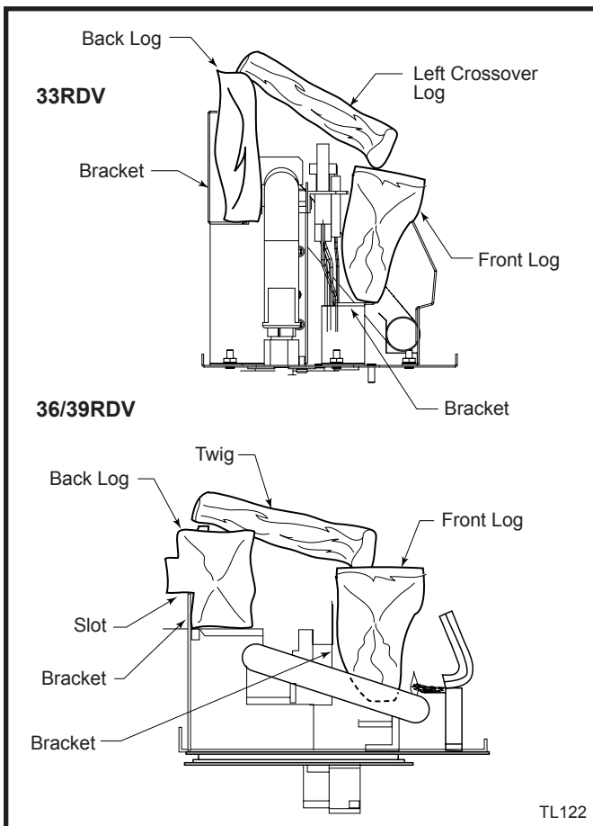
Fig. 43 Side view of logset.
