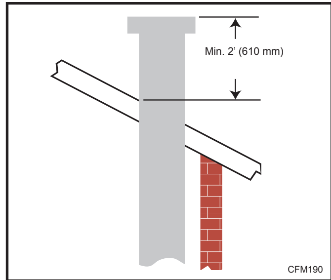
Fig. 37 Minimum termination to roof clearance.
