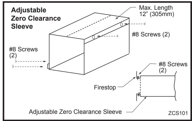
Fig. 23 Adjustable zero clearance sleeve.
