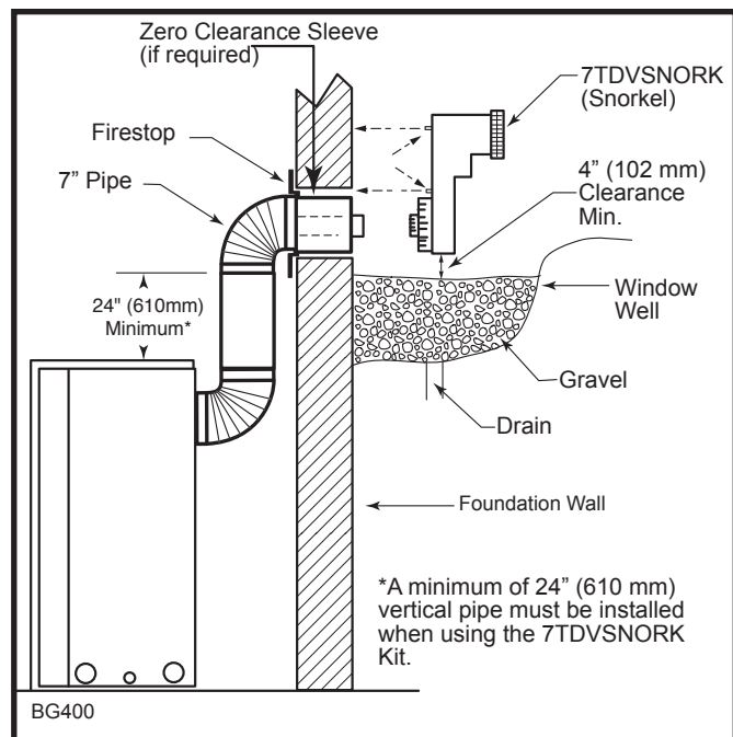
Fig. 30 Below grade installation.
