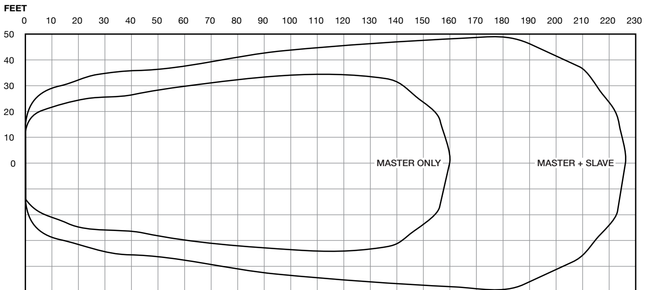
Figure 3: coverage area with second emitter added to same emission point (50% increase)
