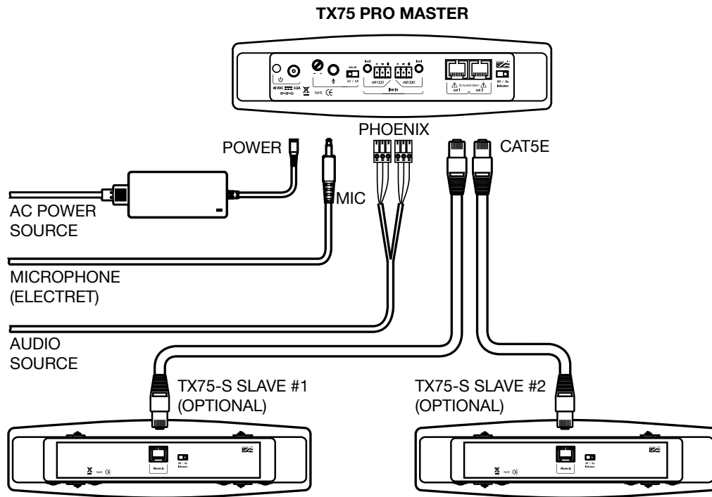
Figure 9: Connecting a WIR TX75 PRO master transmitter to two WIR TX75-S slave emitters
