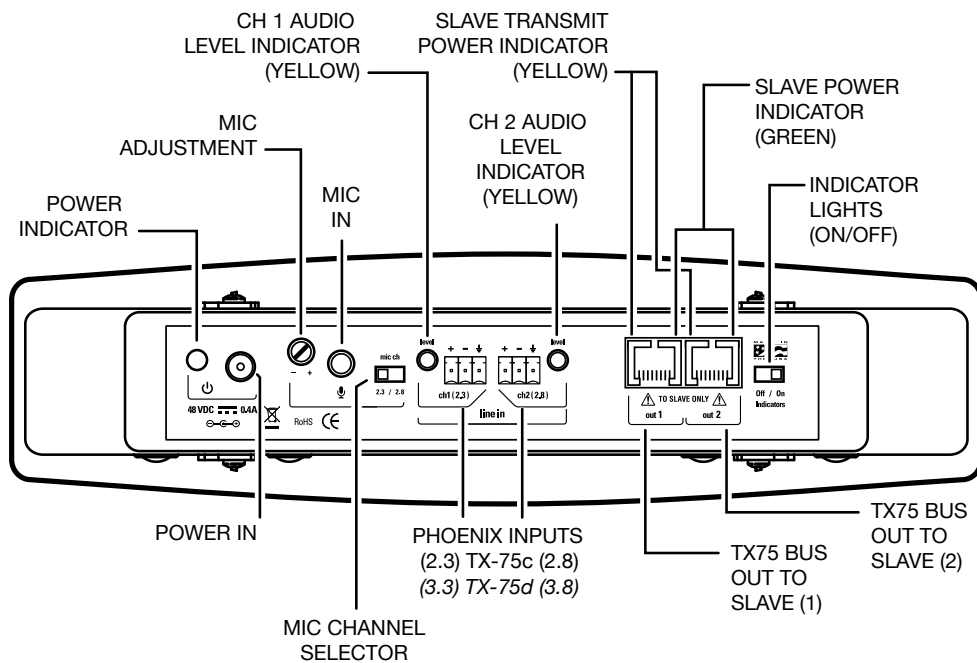
Figure 6: WIR TX75 master rear view
