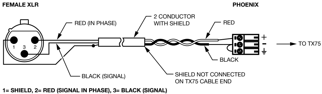
Figure 8: Unbalanced line out (XLR) to WIR TX75 PRO line input (Phoenix) cable
