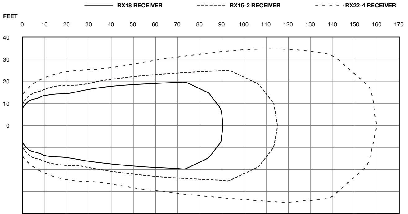
Figure 1: Receiver coverage area with WIR TX75 PRO transmitter OR WIR TX75-S slave emitter in single channel mode.
