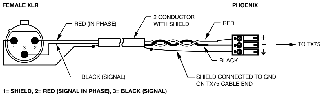
Figure 7: Balanced line out (XLR) to WIR TX75 PRO line input (Phoenix Contact® connector) cable
