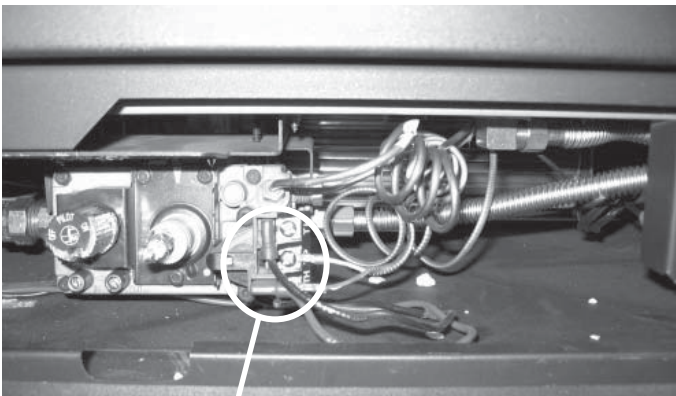
ON/OFF Wires
