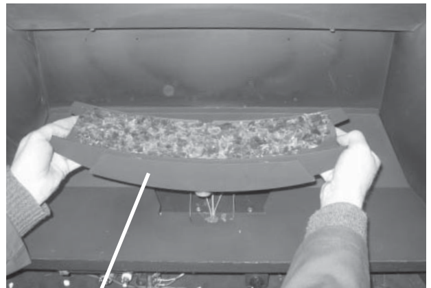
Burner
