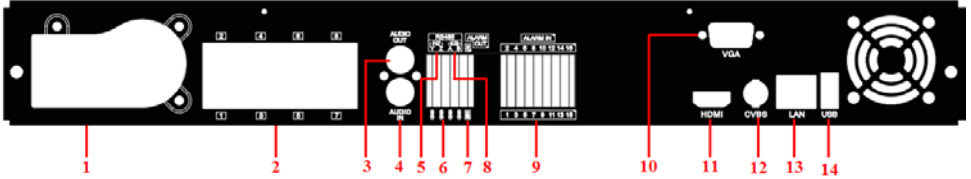
Fig 2-7 Rear Panel for 16-ch
