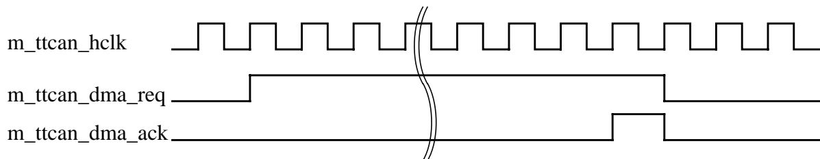
Figure 16 Timing of DMA Interface Signals
