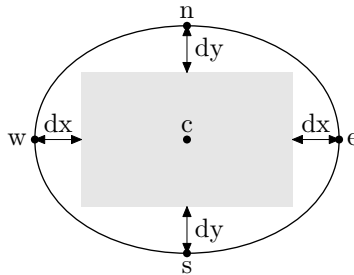
Figure 51: The relationship between the picture given to circleit and the associated variables. The picture is indicated by a gray rectangle.
