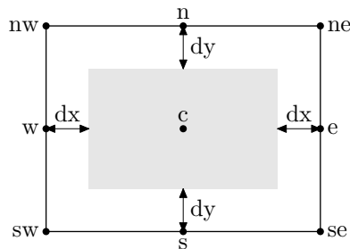
Figure 49: The relationship between the picture given to boxit and the associated variables. The picture is indicated by a gray rectangle.
