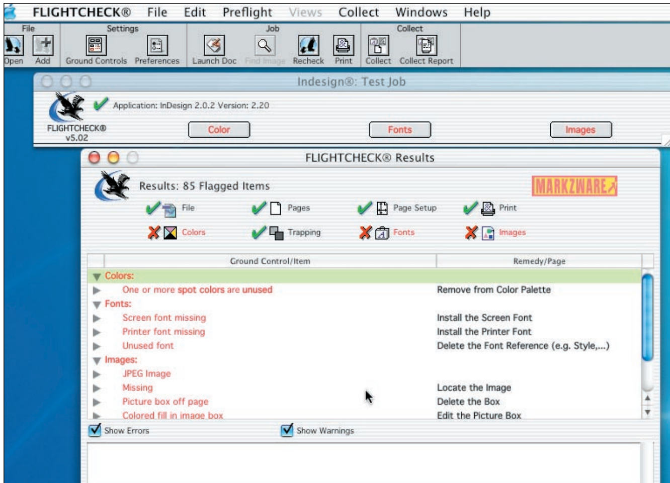
FlightCheck 5 Designer showing (from top to bottom) pull-down menu bar, FlightStrip, Overview window, and Results window.
