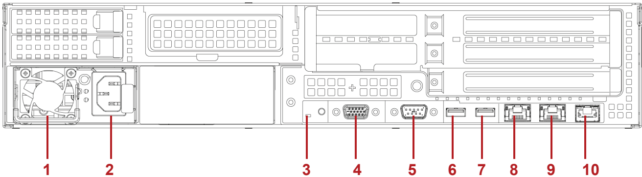
Figure 1-6. System Rear View
