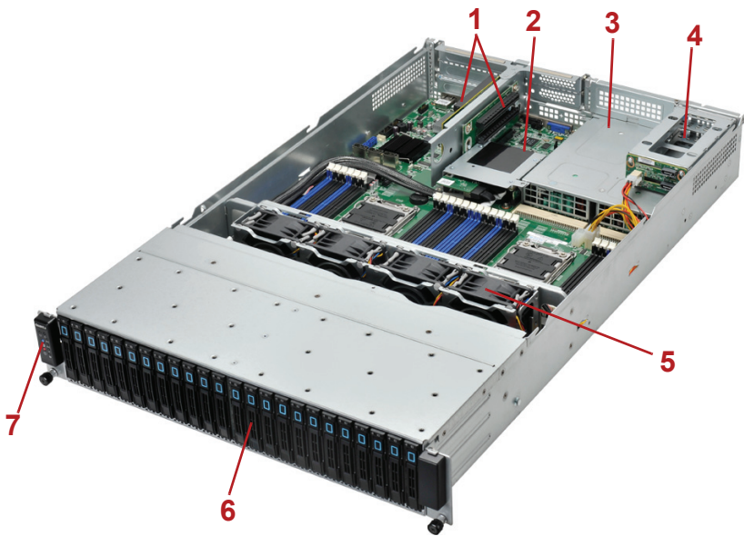
Figure 1-1. 2.5” HDD System Component Overview
