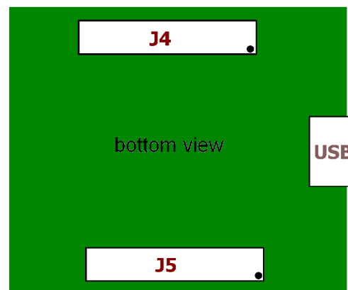
Figure 4: connector receptacles J4 and J5 (bottom view).
