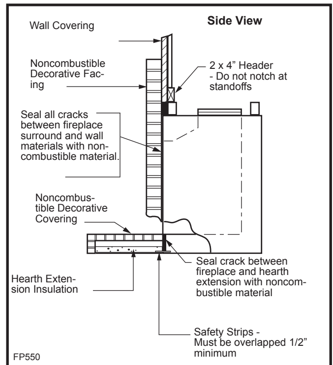
Fig. 23 Sealing gaps.
