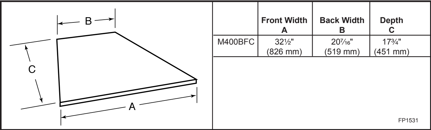
Fig. 1a Hearth dimensions.
