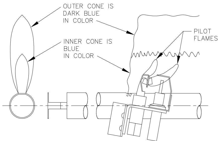
Figure 6: Pilot and Main Burner Flames
