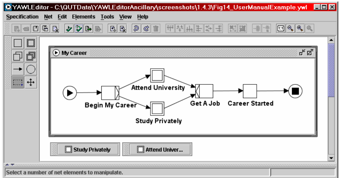
Fig. 15 - Making the "Study Privately " task an atomic composite
