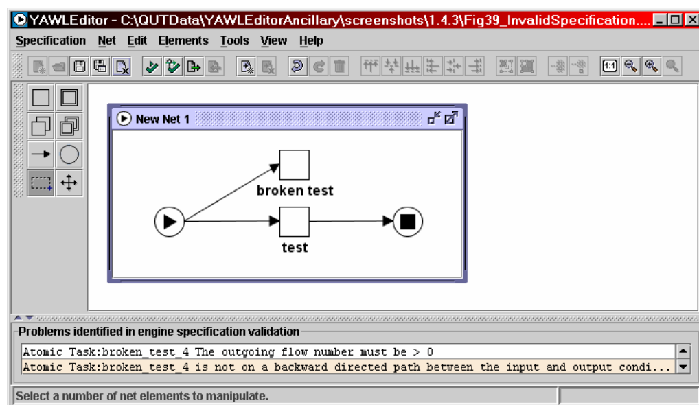
Fig. 39. An invalid specification
