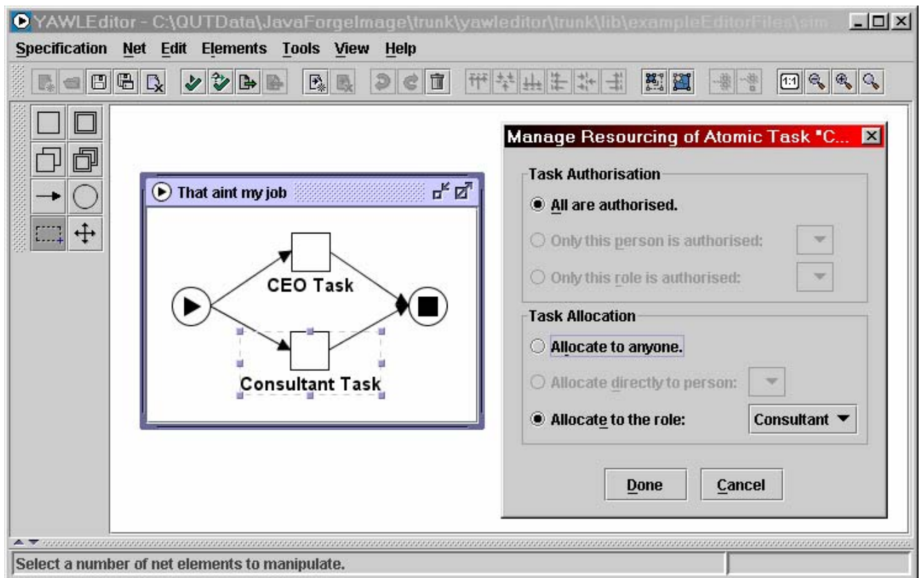
Fig. 47 Managing Resourcing of a task
