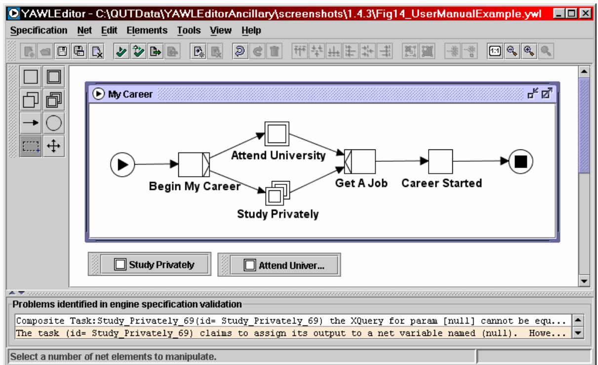
Fig. 14 - Validation with unfinished Multiple-Instance Tasks
