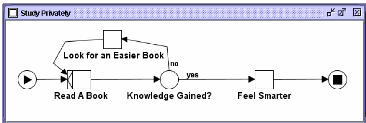
Fig. 17. Adding “knees” to a Flow Relation
