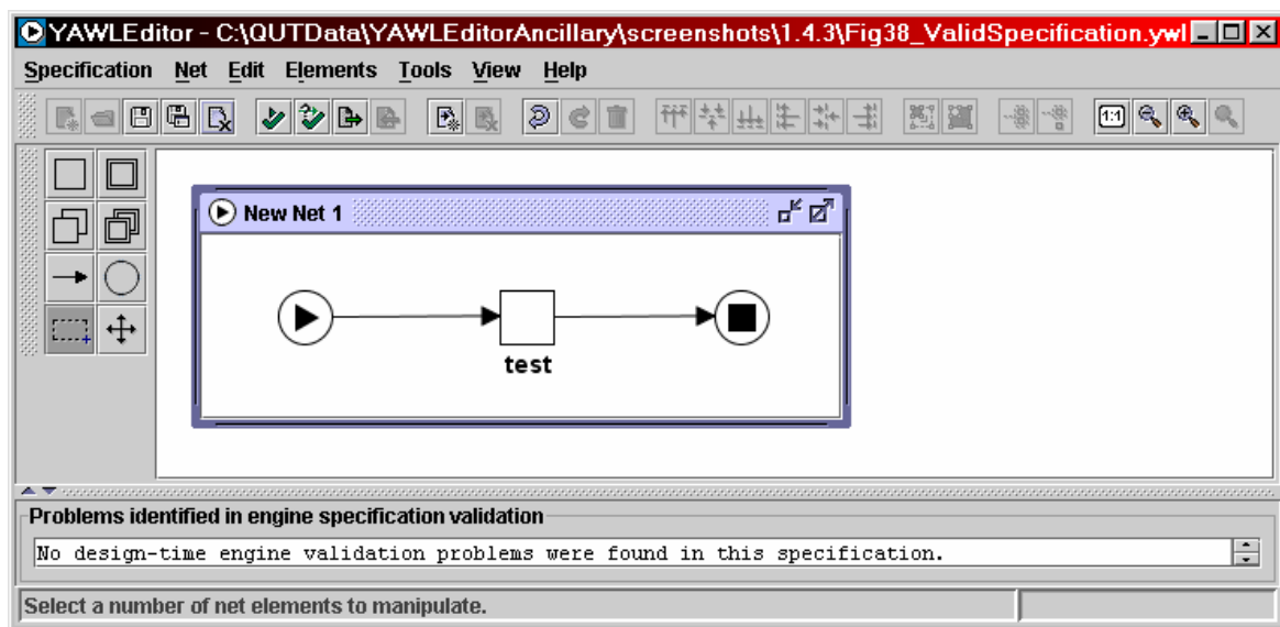
Fig. 38. A valid specification
