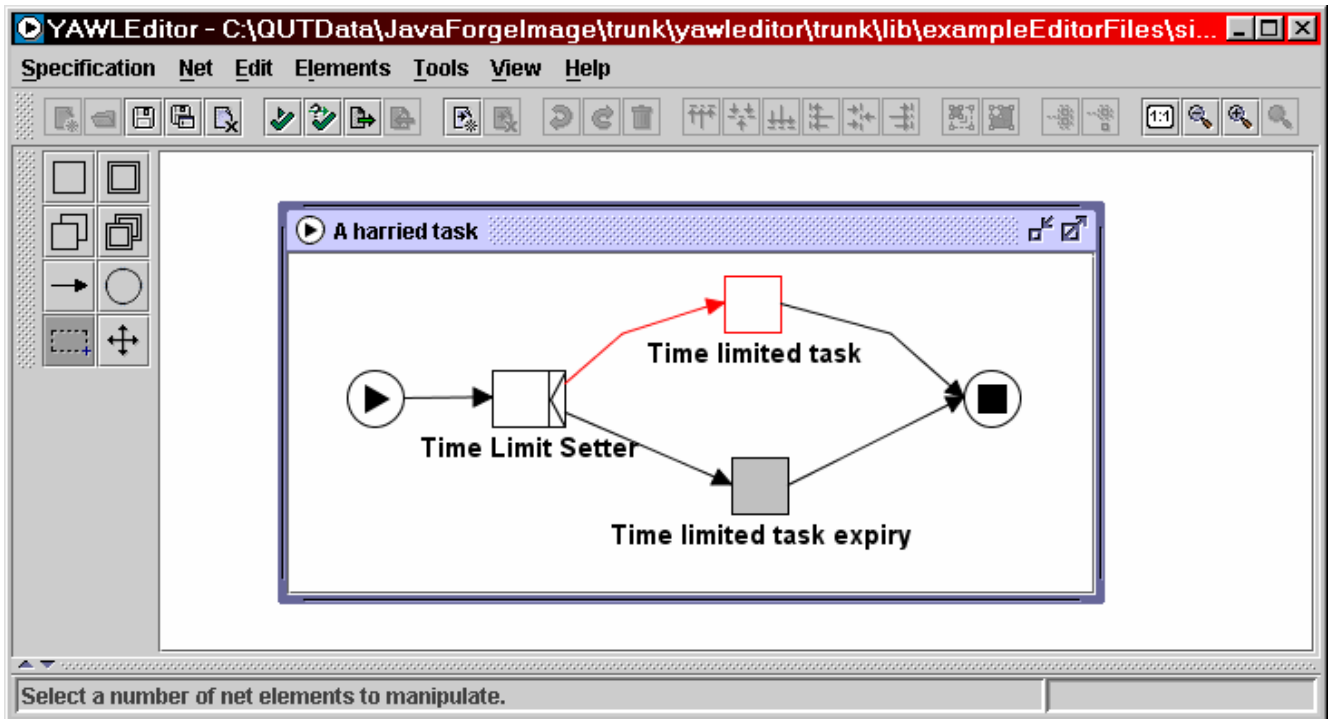
Fig. 45 - Example showing the usage of a custom YAWL service
