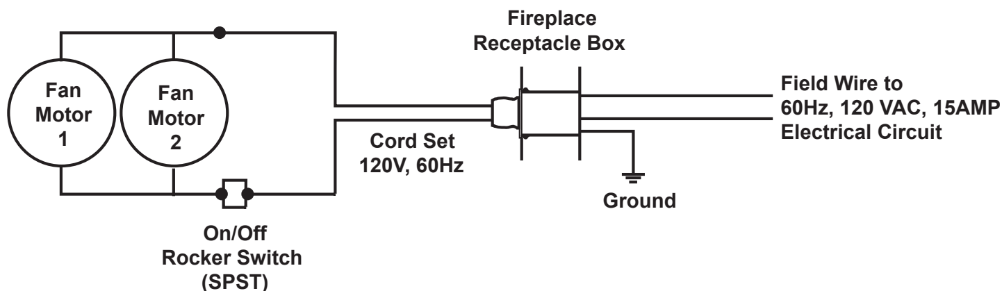
Figure 26 - Wiring Diagram
