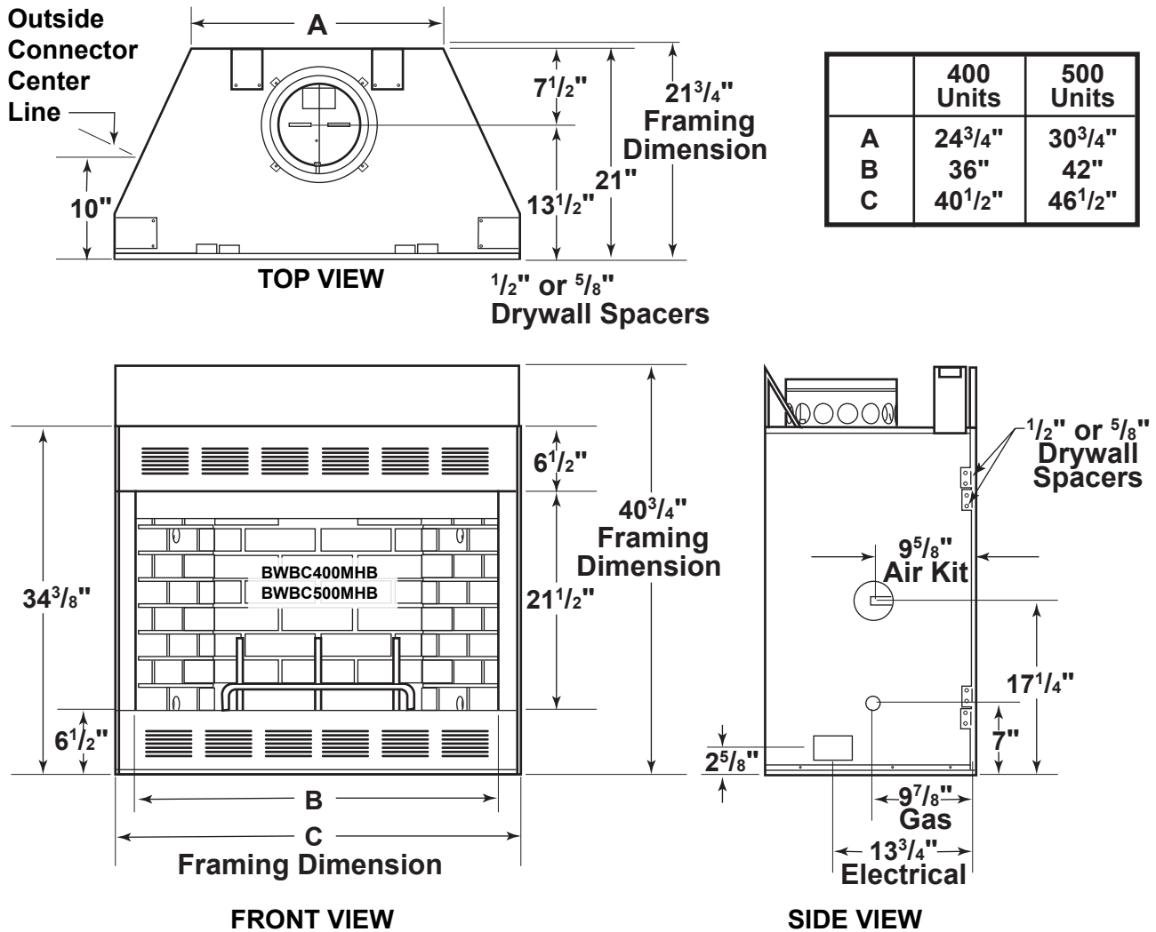
Figure 7 - Fireplace Dimensions
