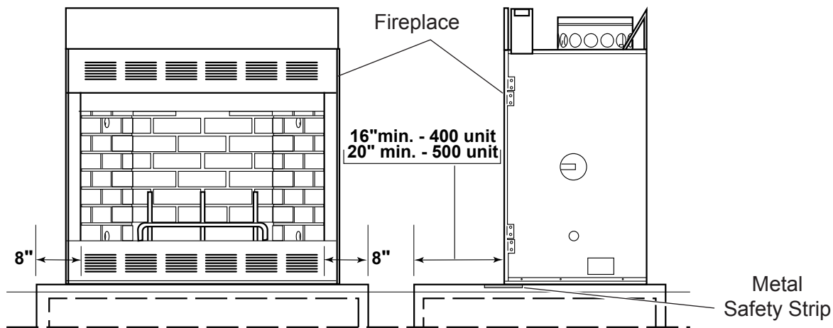
Figure 9 - Installing Hearth Extension and Metal Safety Strip
