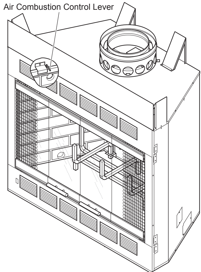
Figure 5 - Outside Combustion Air Control Lever Location
