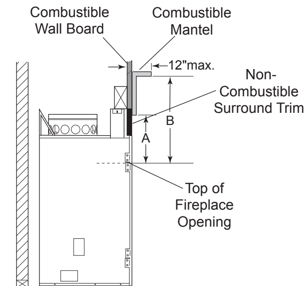
Figure 25 - Locating Mantel
