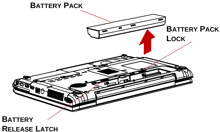
Figure 6-2 Removing the battery pack
