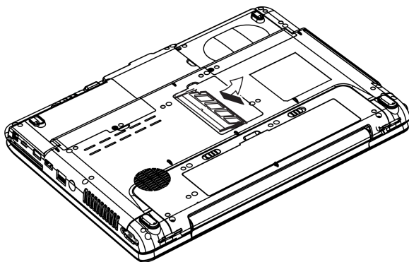
Figure 8-6 Inserting the memory module
