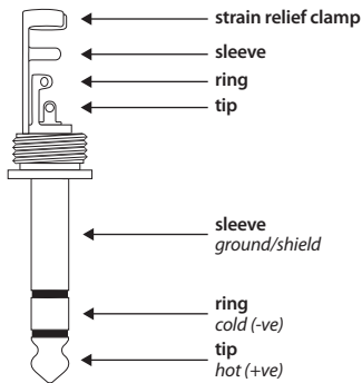
Fig. 3.2: 1/4" TRS connector
