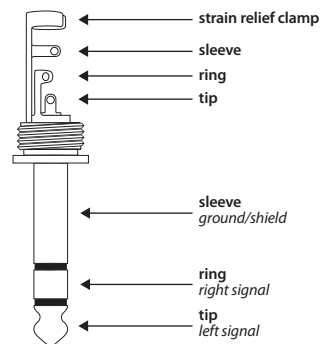
Fig. 3.5: 1/4" headphones connector
