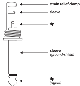
Fig. 3.3: 1/4" TS connector
