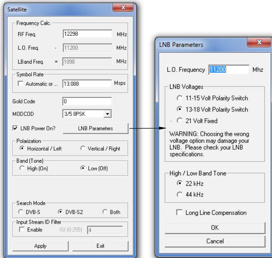
Figure 8: Satellite Configuration and LNB Parameters Dialog
