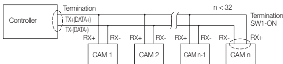
<RS-485 Half Duplex Organization>
