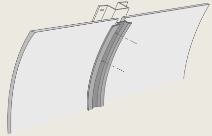
Fixing of flat enamel panels in a tunnel. High-quality stainless steel sub-frame
