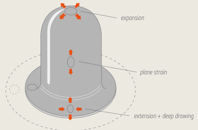
Different deformation modes in a drawn component
