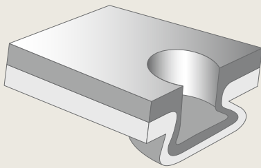
Clinched joint
