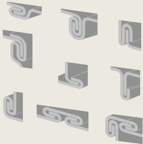
Different single and double lock seams
