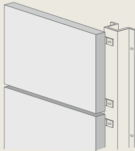
Sub-frame in hot dip galvanised steel or stainless steel, variable joints, enamel panels 1.5 mm thick plus backing board
