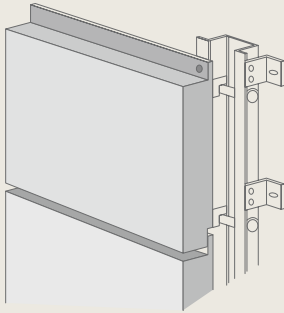
Fixing of a rainscreen cladding
