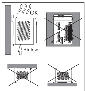
Mounting orientation
