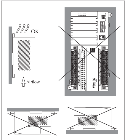
Mounting orientation
