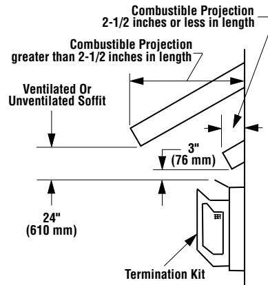
Figure 6 - Side Elevation View
