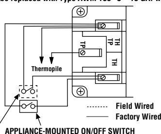
Millivolt Wiring Diagram
