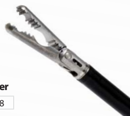
5 mm Crocodile Grasper
