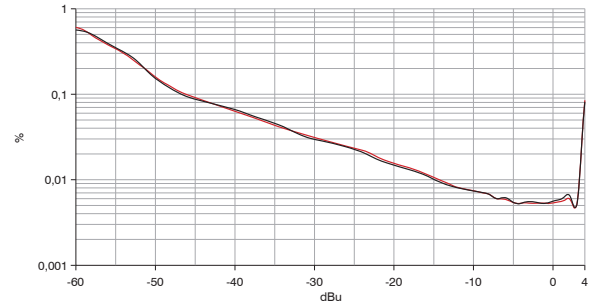
Figure 7.3 THD @ 1 kHz vs. input level @ 2 Ω load (32 dB amplifier gain) (Measurement of a typical performance of Ch 1 & Ch 2)
