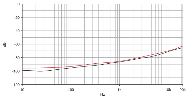
Figure 7.5 Channel separation vs. frequency @ 120 W/4 Ω (Measurement of a typical performance of Ch 1 → Ch 2 & Ch 2 → Ch 1)
