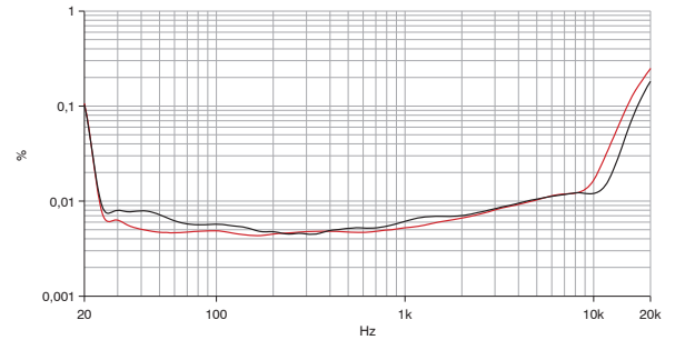
Figure 7.4 THD vs. frequency, 120 W output power (Measurement of a typical performance @ 2 Ω & 4 Ω)
