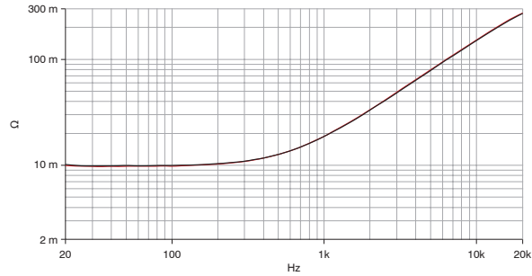
Figure 7.9 Output impedance vs. frequency @ 1 Amp RMS injected current equivalent 11\text{ m}\Omega + 2,1\text{ }\mu\text{H} (Measurement of a typical performance of Ch 1 & Ch 2)
