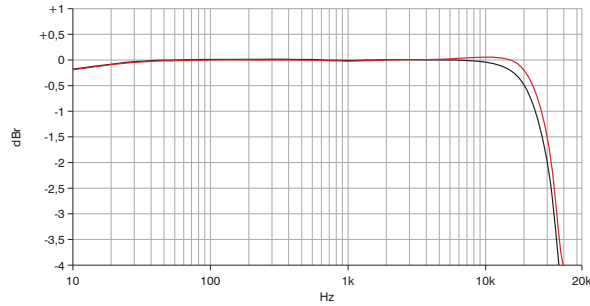
Figure 7.1 Gain vs. frequency, 120 W output power (Measurement of a typical performance @ 2 Ω & 4 Ω)
