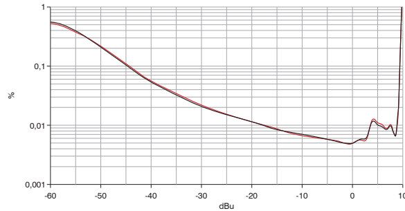
Figure 7.2 THD @ 1 kHz vs. input level @ 4 Ω load (32 dB amplifier gain) (Measurement of a typical performance of Ch 1 & Ch 2)
