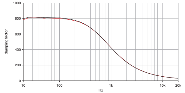
Figure 7.10 Damping factor into 8\text{ }\Omega Damping factor = loaded impedance / amplifier output impedance (equation: damping factor = loaded impedance / amplifier output impedance) (Measurement of a typical performance of Ch 1 & Ch 2)
