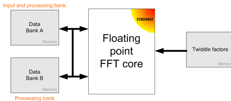
Figure 1 : Minimum memory usage architecture
