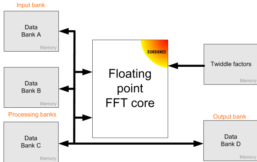
Figure 2 : Streaming IO memory architecture
