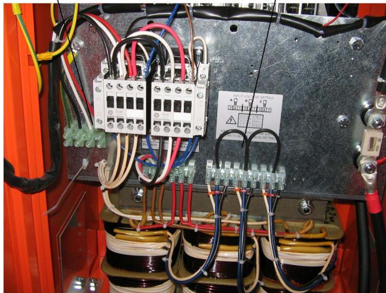
POWER TRANSFORMER TAPS
