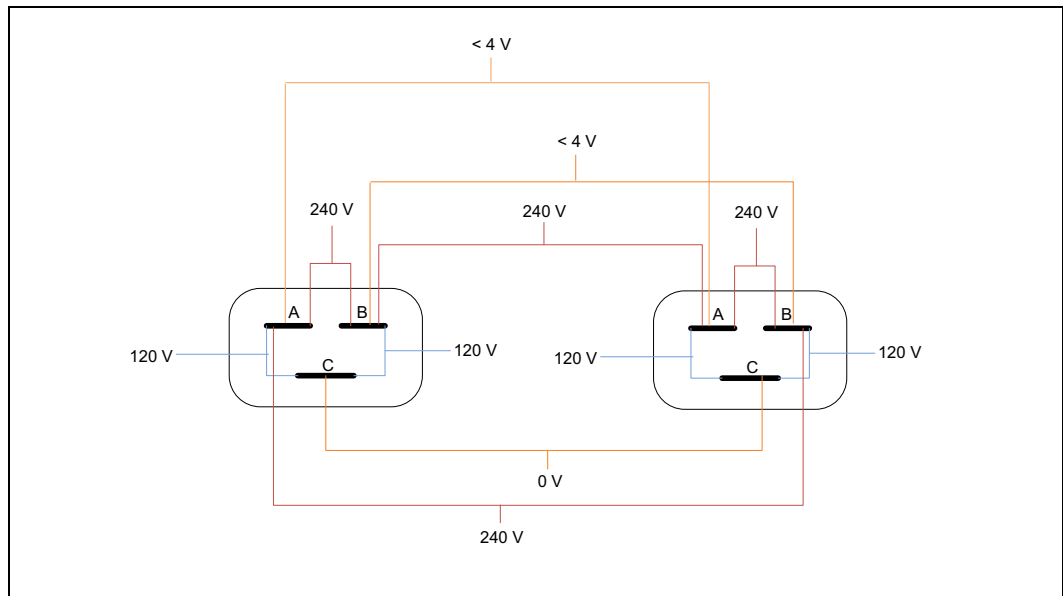
Figure 10 Dual AC input voltage requirements.
