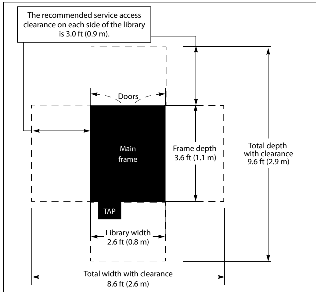
Figure 6 Dimensions of a single-frame T950, including recommended service access clearance.
