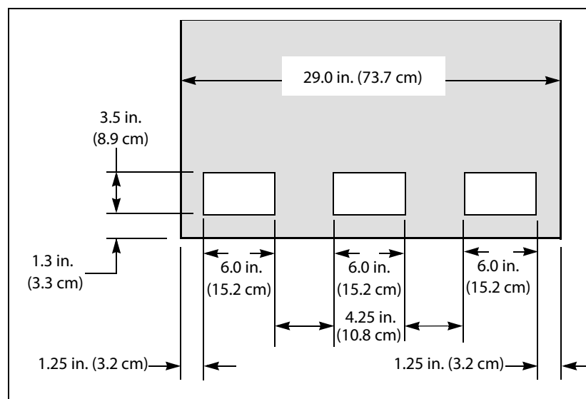
Figure 9 Floor cable access for main and drive expansion frames.
