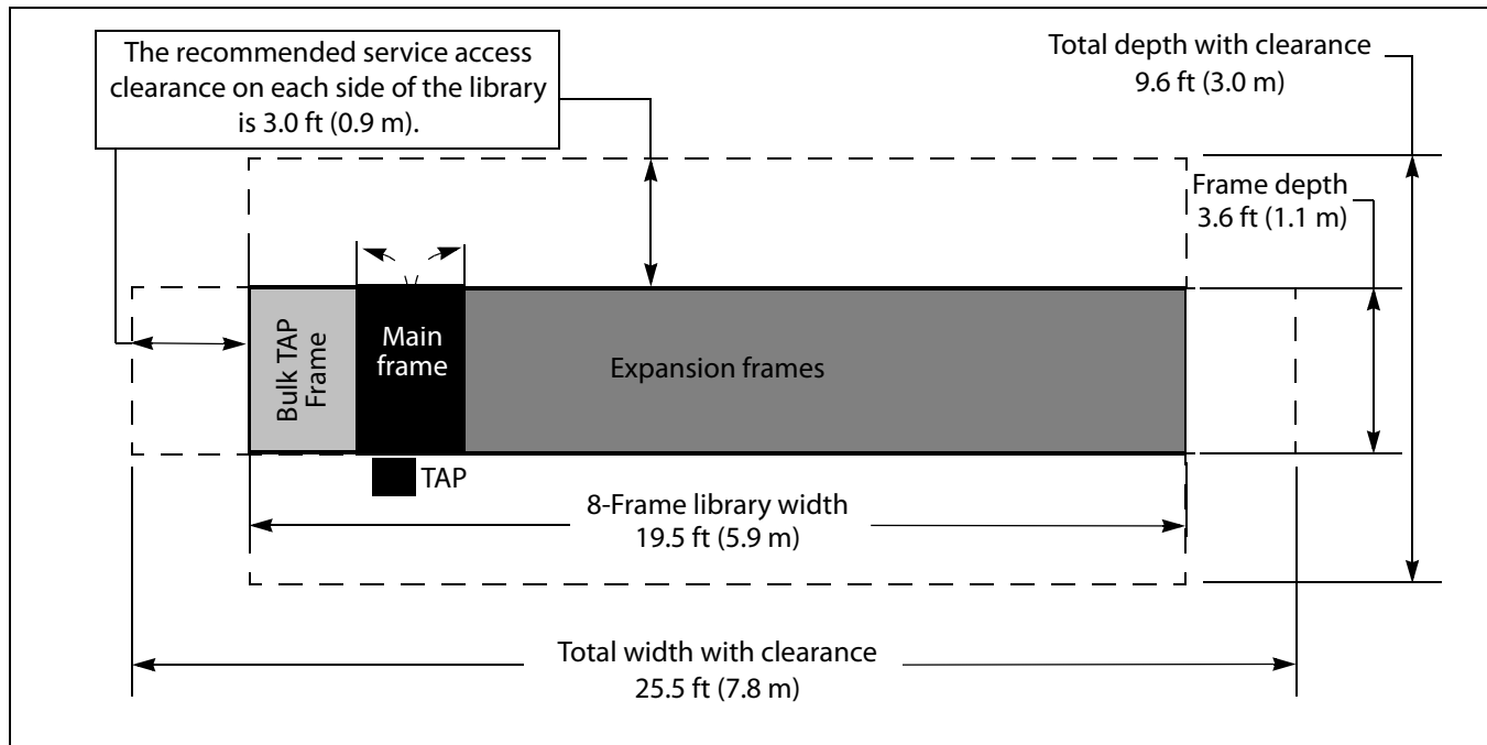
Figure 7 Dimensions of the eight-frame T950, including recommended service access clearance.
