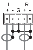
Figure 4: Connecting the Unbalanced Stereo Audio Input
