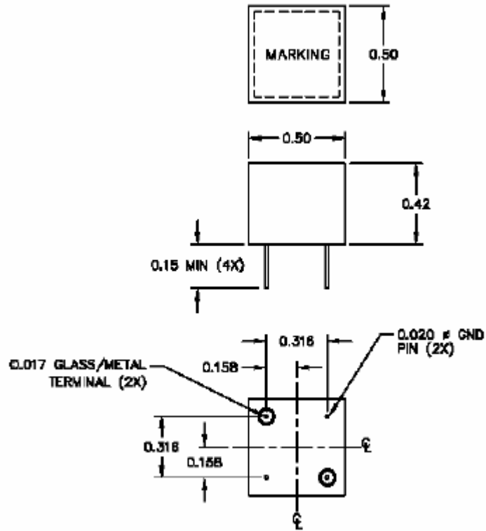
FIGURE-1 DIMENSIONAL DRAWING
