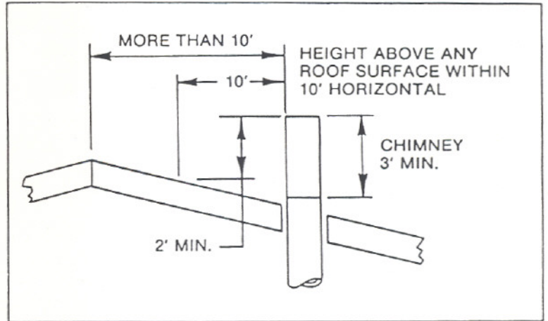
Figure 10 Chimney Height
