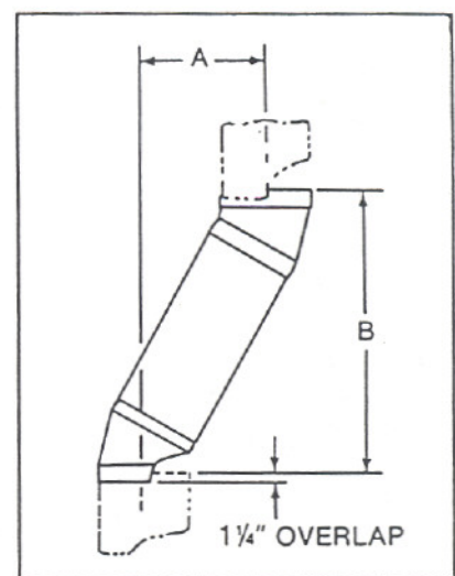
Figure 12 Chimney Offset/ Return
