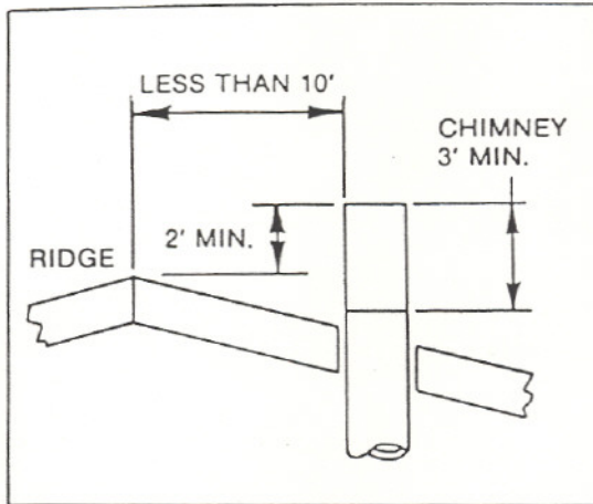
Figure 9 Chimney Height
