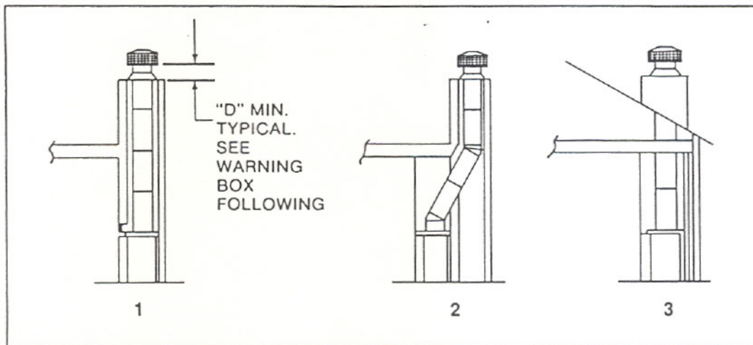
Figure 22 Chase Constructions
