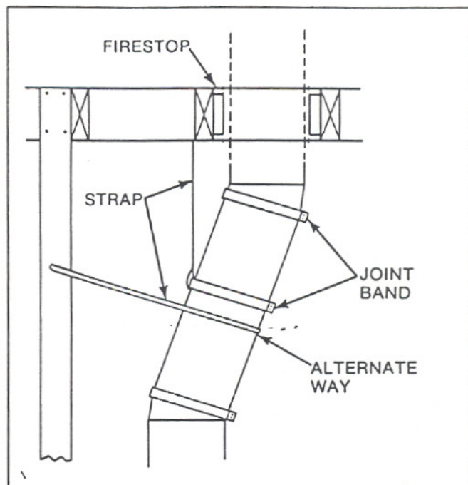
Figure 19 Offset/Return Installation
