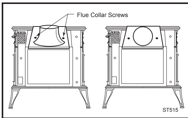
Fig. 30 Reversing the flue collar.
