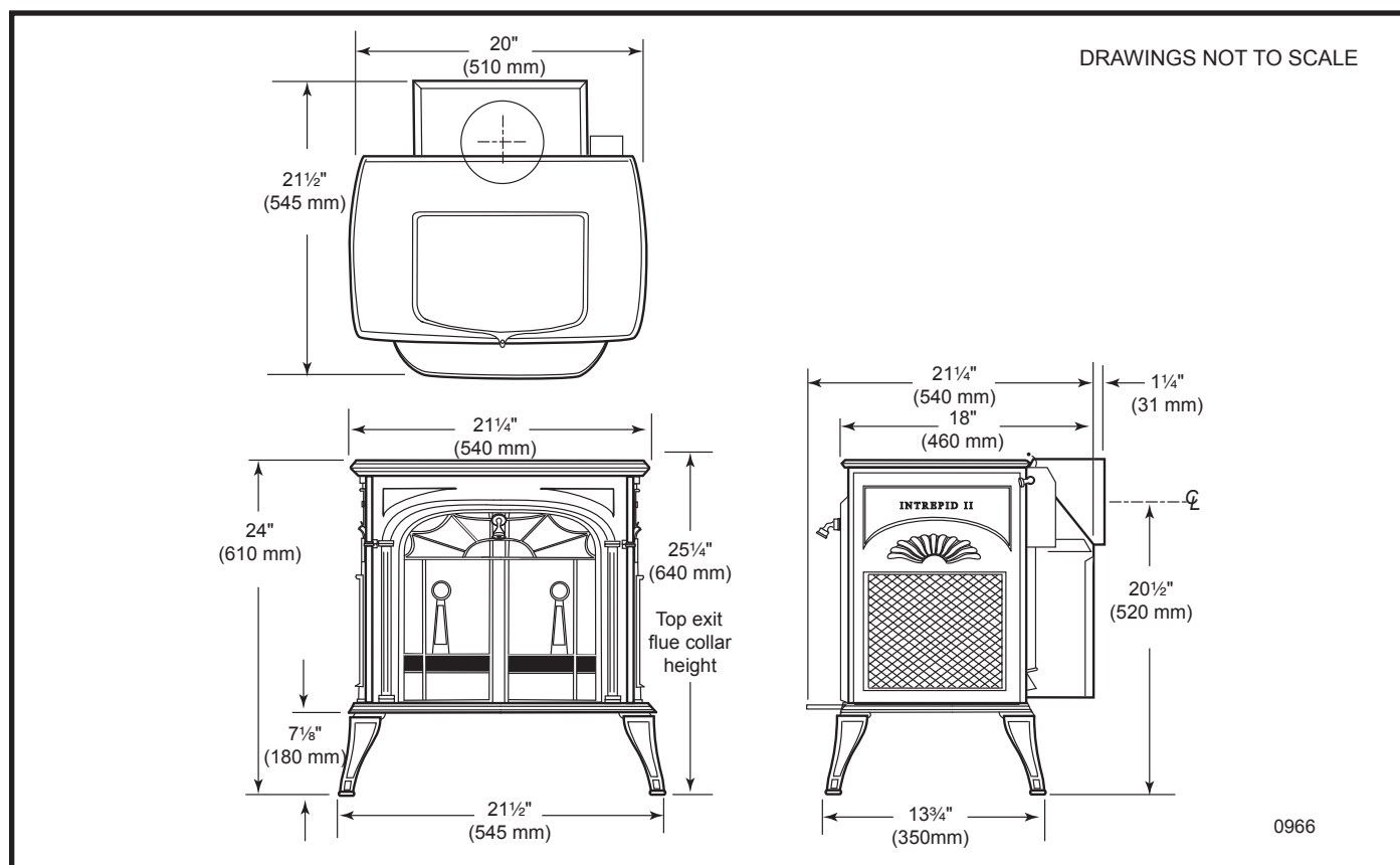
Fig. 1 Intrepid II 1990 dimensions.
