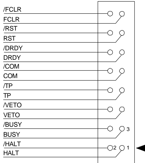
Fig. 2.2: CONTROL connector pin assignment
