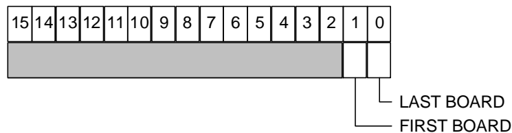
Fig. 3.18: MCST Address Register
