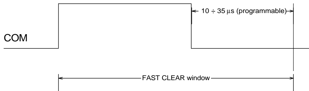
Fig. 5.5: Fast Clear window
