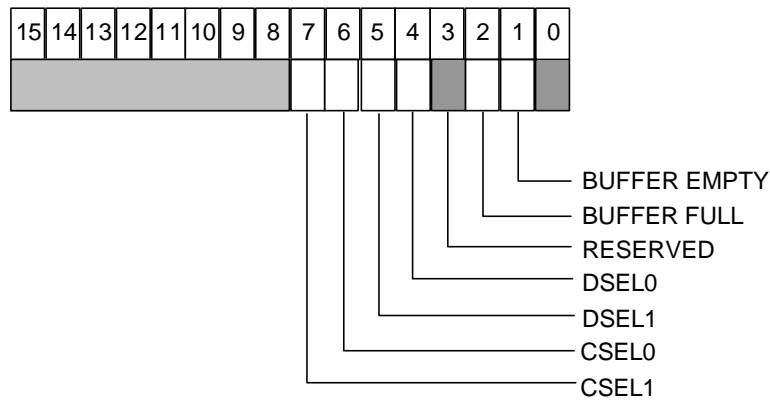
Fig. 3.20: Status Register 2
