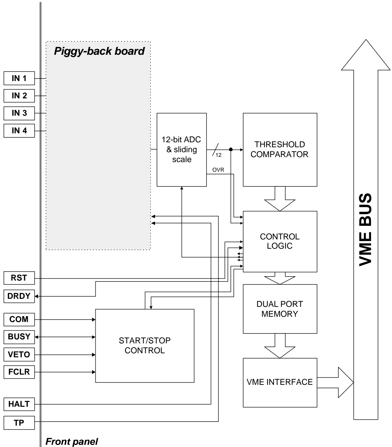
Fig. 1.1: Model V874A Block Diagram
