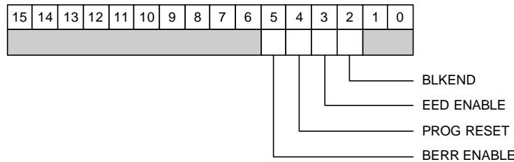
Fig. 3.16: Control Register 1
