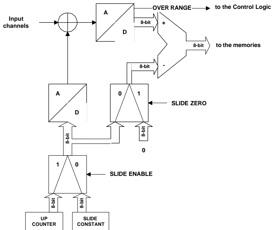
Fig. 5.2: Block diagram of the sliding scale section
