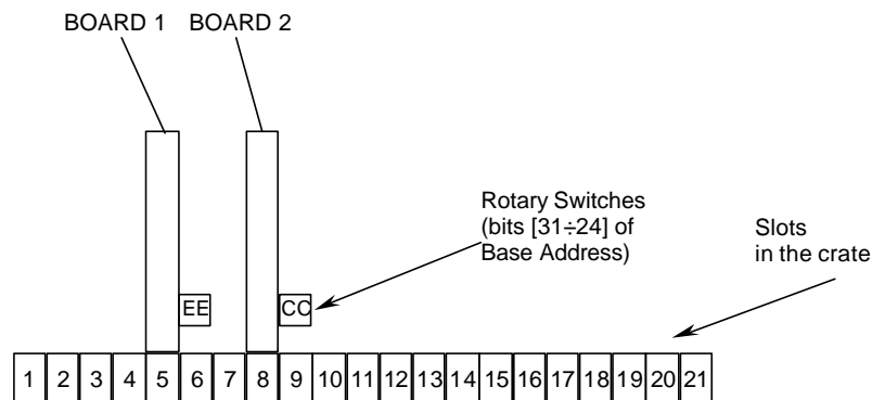
Fig. 3.3: Base/GEO Addressing: Example 1
