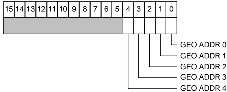
Fig. 3.10: Geographical address register
