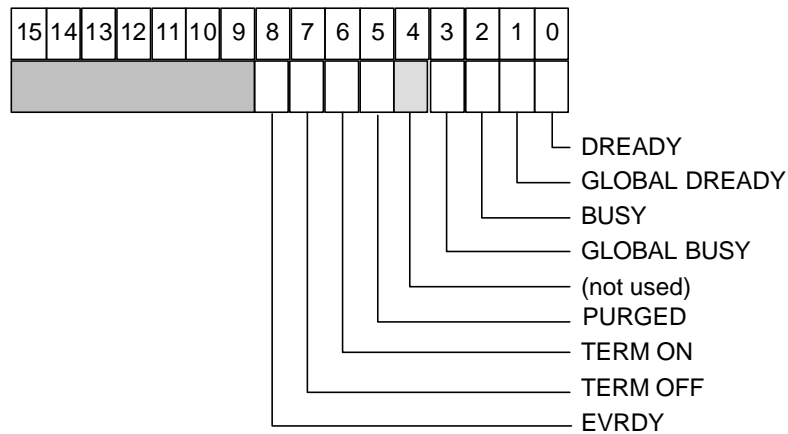
Fig. 3.15: Status Register 1
