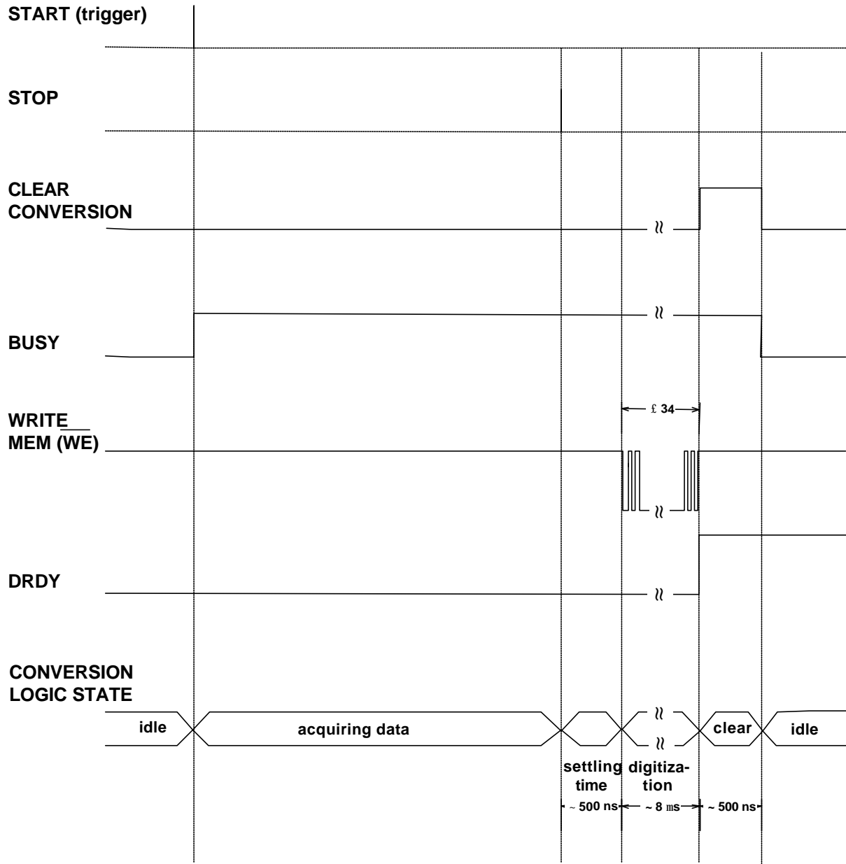
Fig. 5.1: Signal timing for signal conversion
