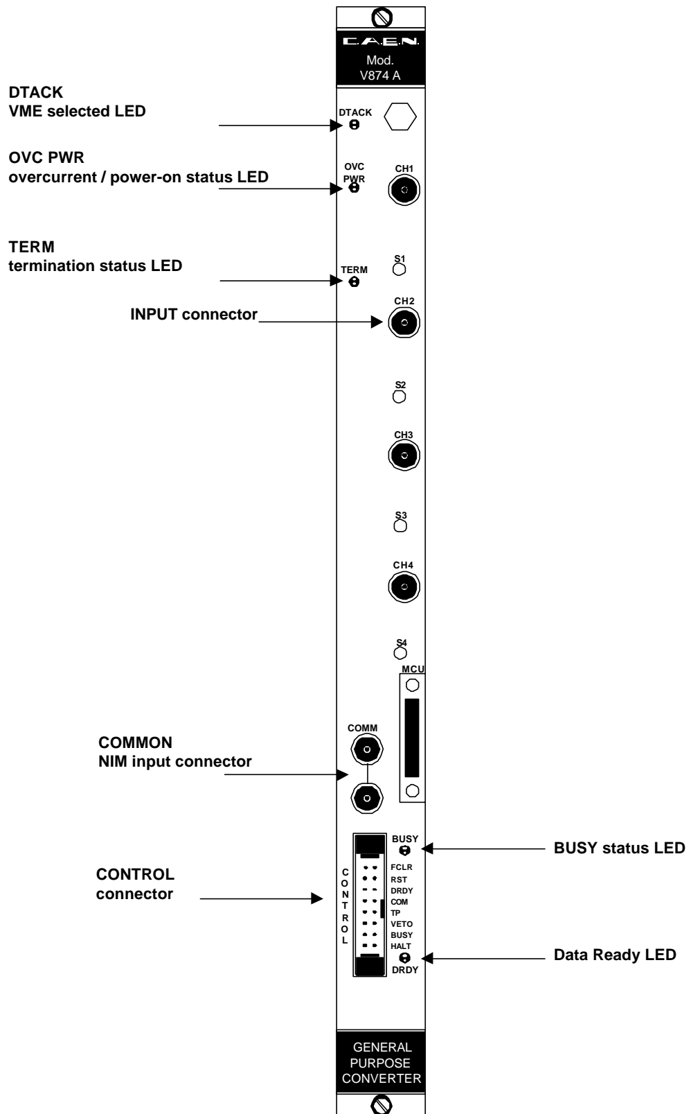
Fig. 2.1: Model V874 A front panel
