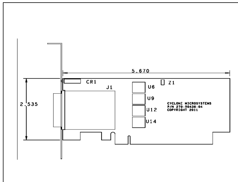
Figure 5-5. PCIe-436 Physical Configuration
