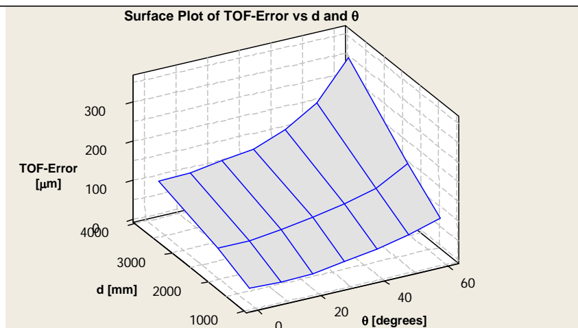
Fig. 4.10. Surface plot to represent the effect of the interaction of factors d and \theta on the TOF-Error
