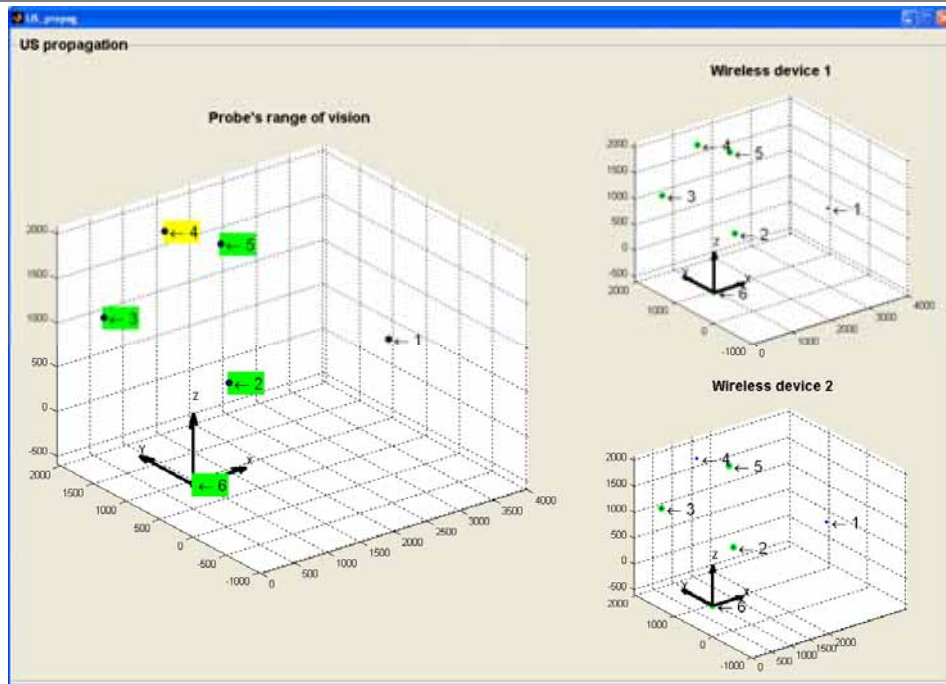
Fig. 5.3. Graphic representation of the probe range of vision. The right part of this screenshot shows the constellation devices seen by the mobile probe Crickets
