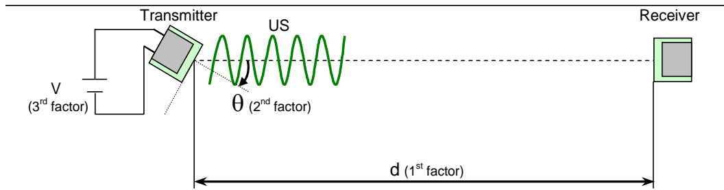
Fig. 4.5. Experimental setup
