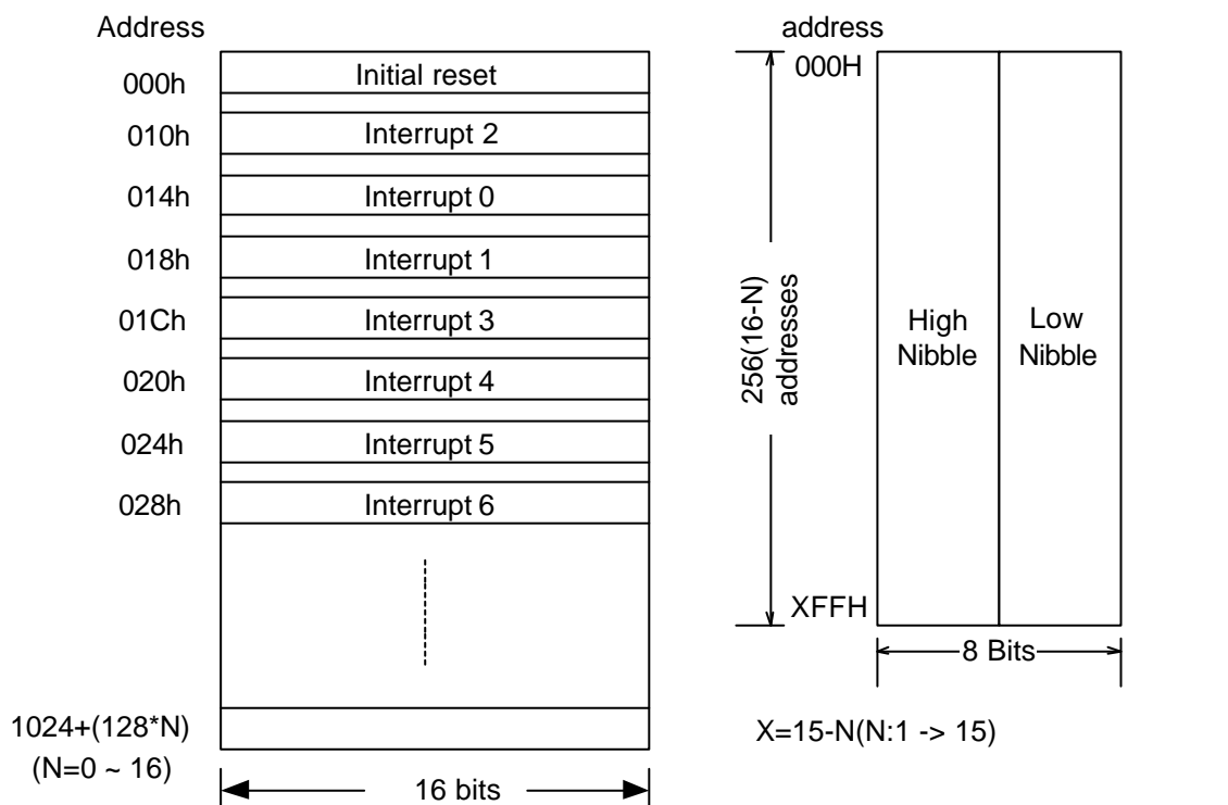
Instruction ROM ( PROM ) organization
