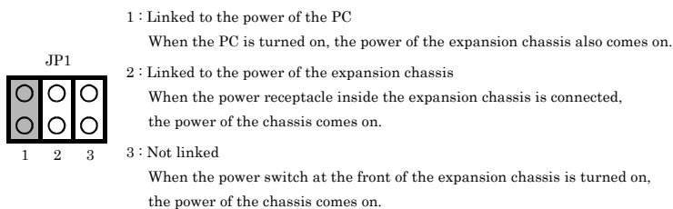
Figure 2.3. Setting Jumper
