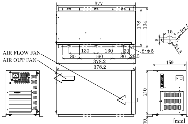
Figure 3.2. Physical Dimensions < ECH-PE-CE-F4A, Vertically placed >
