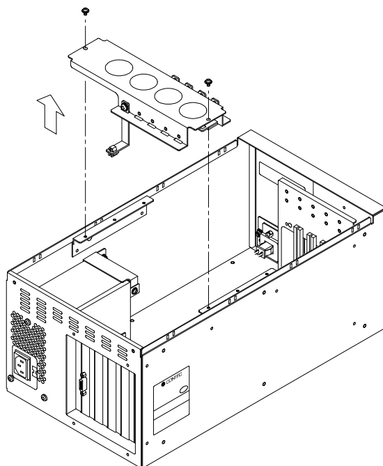
Figure 2.5. Removing the fall-off prevention bar
