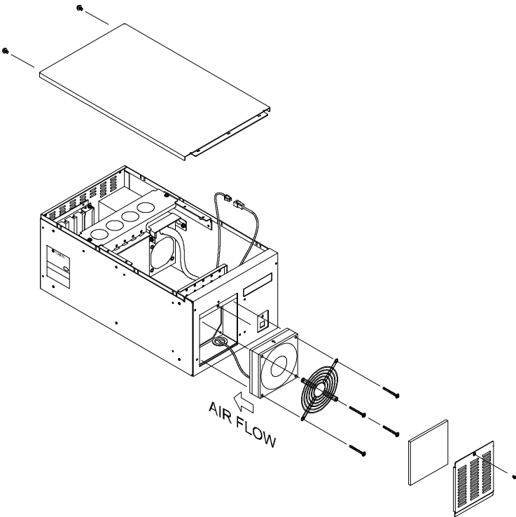
Figure 2.12. Installing/Removing a fan and filter
