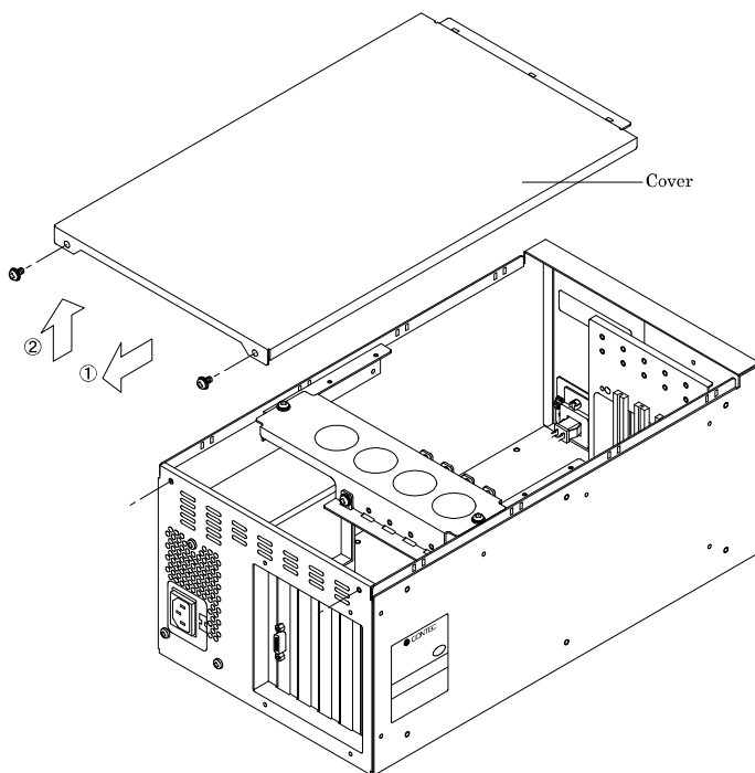
Figure 2.4. Removing the cover
