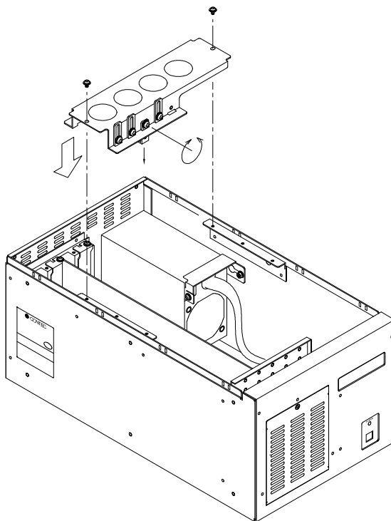
Figure 2.7. Attaching the fall-off prevention bar
