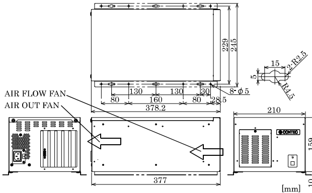
Figure 3.1. Physical Dimensions < ECH-PE-CE-F4A, Horizontally placed >
