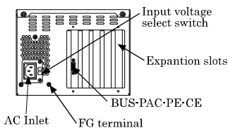
Figure 2.2. Names of major parts < ECH-PE-CE-F4A >
