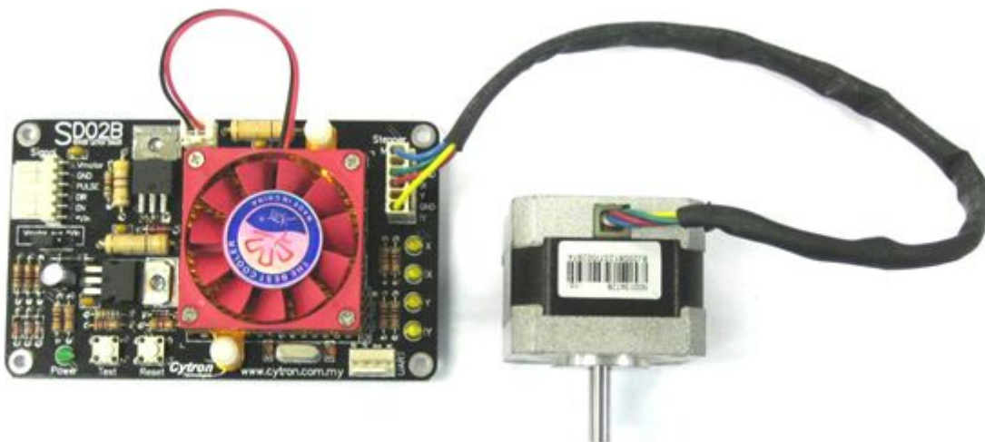
Bipolar Stepper motor (4 wires)
