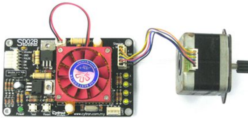
Unipolar Stepper motor (6 wires)
