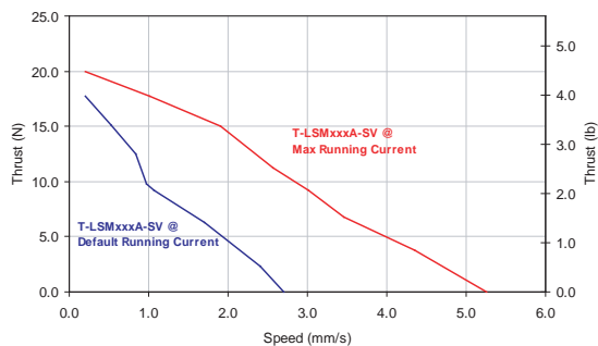
T-LSMxxxA-SV Performance
