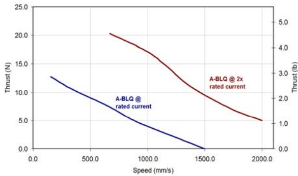
A-BLQ Performance
