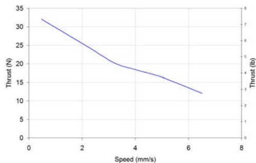
T-LS Performance
