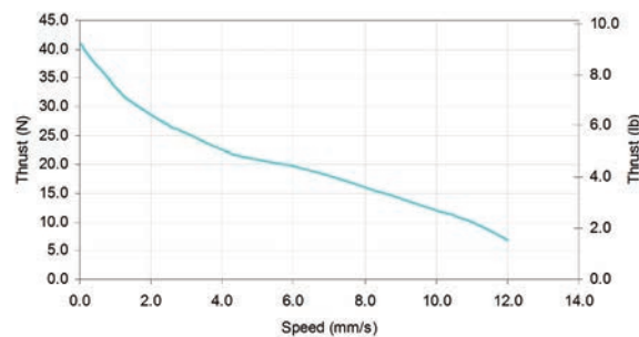
LAC10A Performance Curve at 24V
