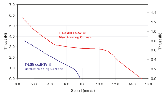
T-LSMxxxB-SV Performance
