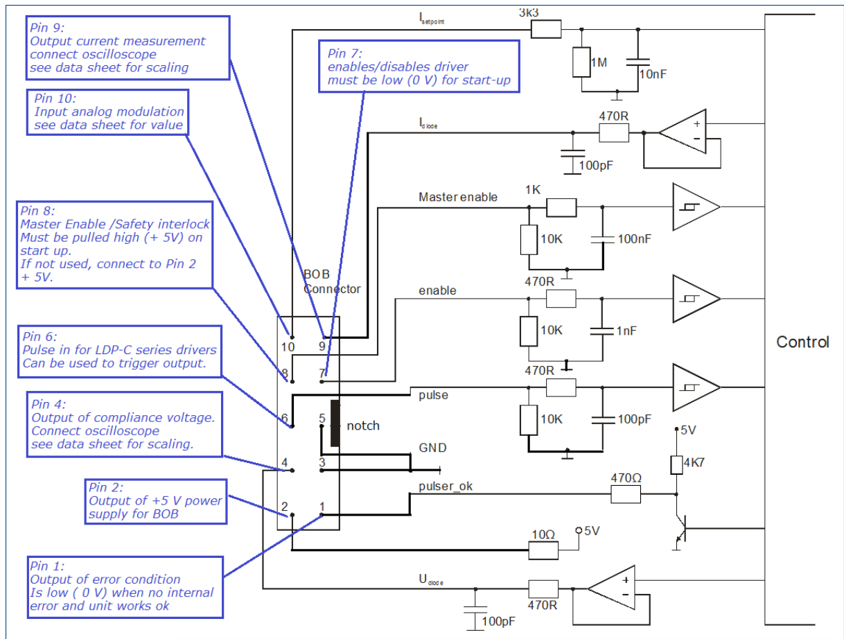
Functional Description of BOB-Connector Interface
