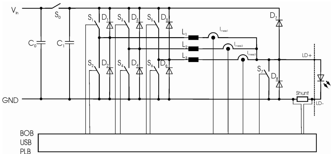
Operation Principle of LDP-C 120-20 driver
