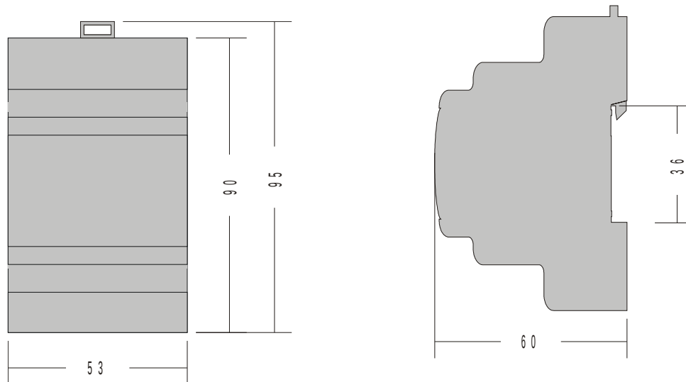
Figure 3: Housing dimensions
