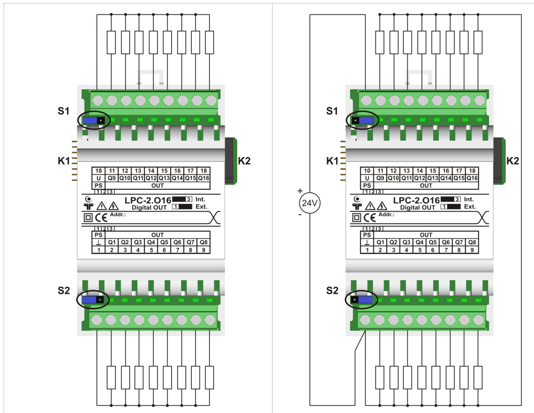
Figure 2: Connection scheme
