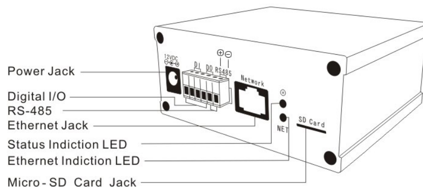
Figure 2-2: Major components in the back panel
