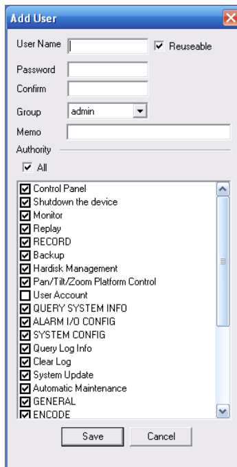
Figure 5-42 Add user
