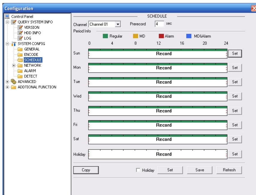
Figure 5-21 Schedule
