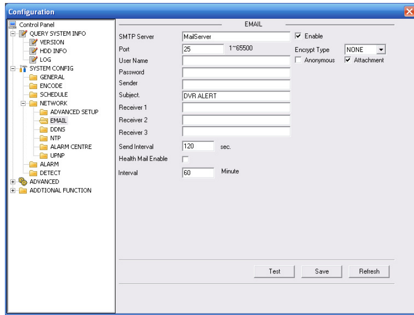
Figure 5-27 Email
