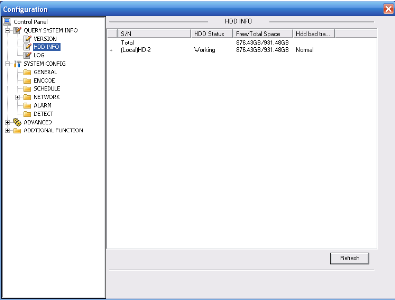
Figure 5-15 HDD Information
