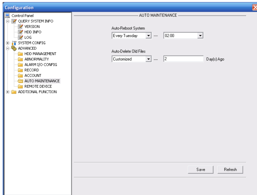
Figure 5-43 Auto Maintenance
