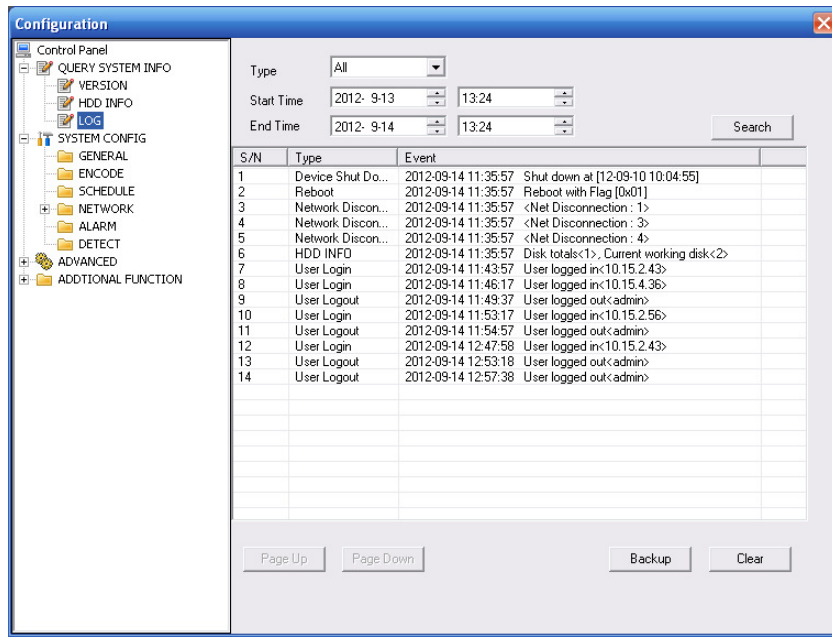
Figure 5-16 Log
