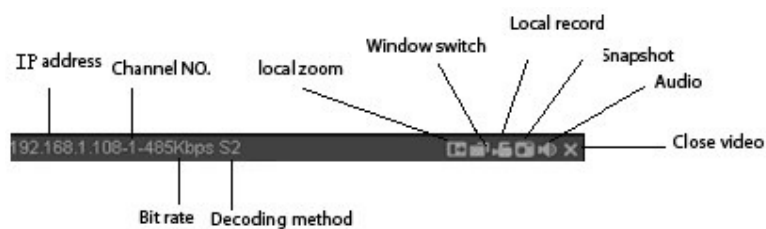
Figure 5-6 Real-time Monitor
