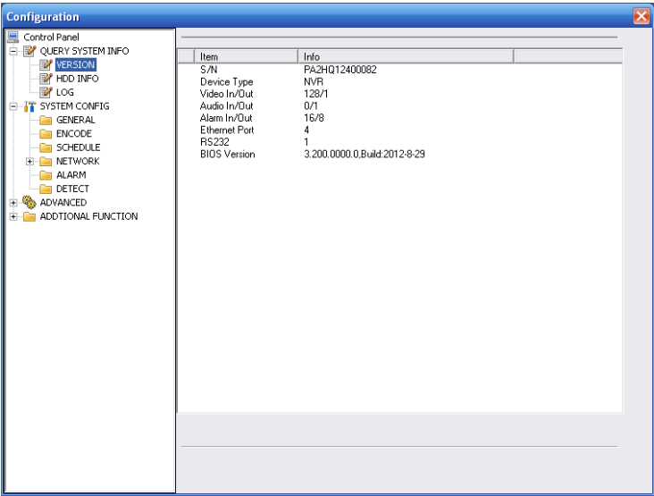
Figure 5-14 Version Information
