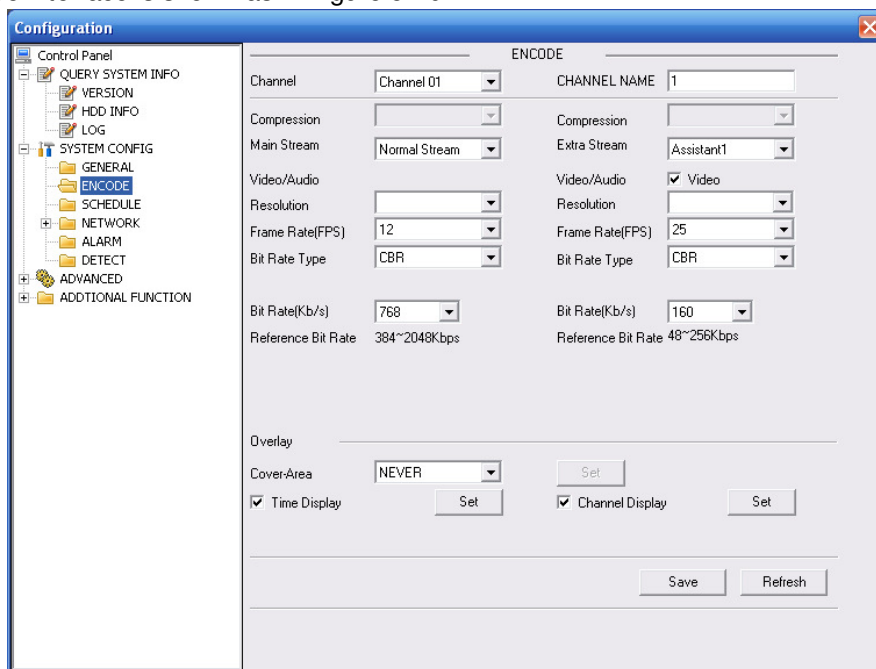
Figure 5-20 Encode
