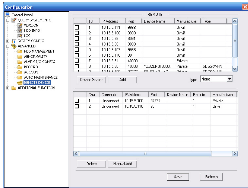
Figure 5-44 Remote device
