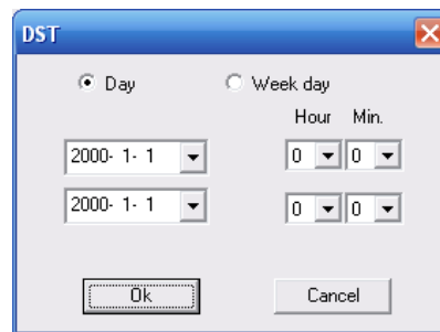
Figure 5-18 DST
