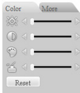
Figure 5-12 Color
