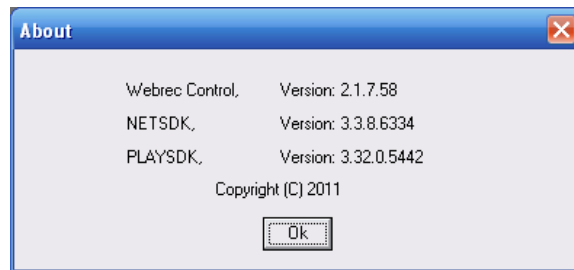
Figure 5-52 About
