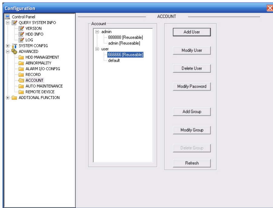
Figure 5-41 Account
