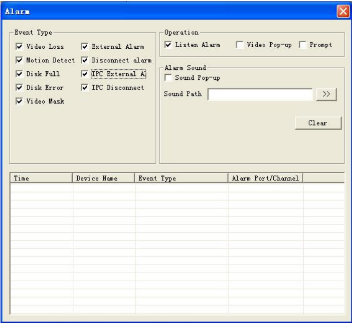
Figure 5-51 Alarm
