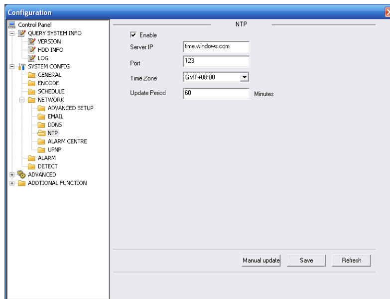
Figure 5-29 NTP
