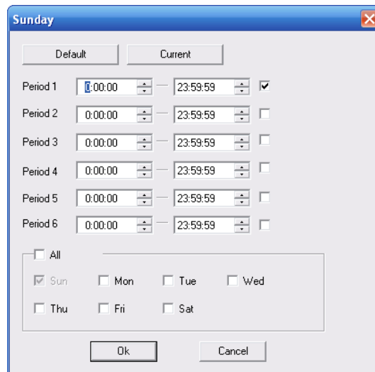
Figure 5-34
