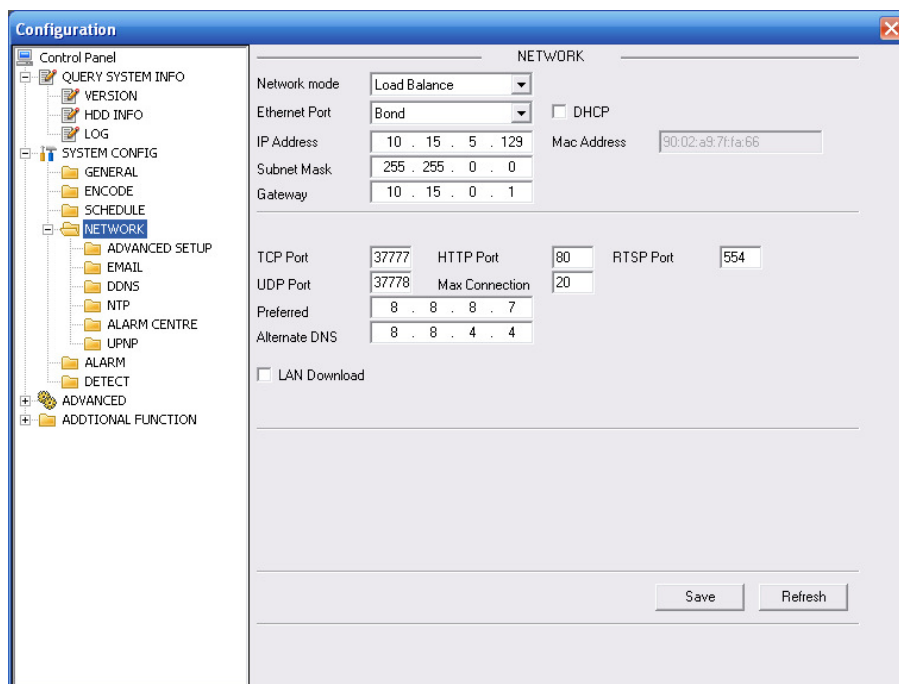
Figure 5-25 Network
