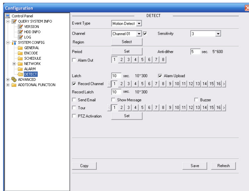
Figure 5-35 Detect
