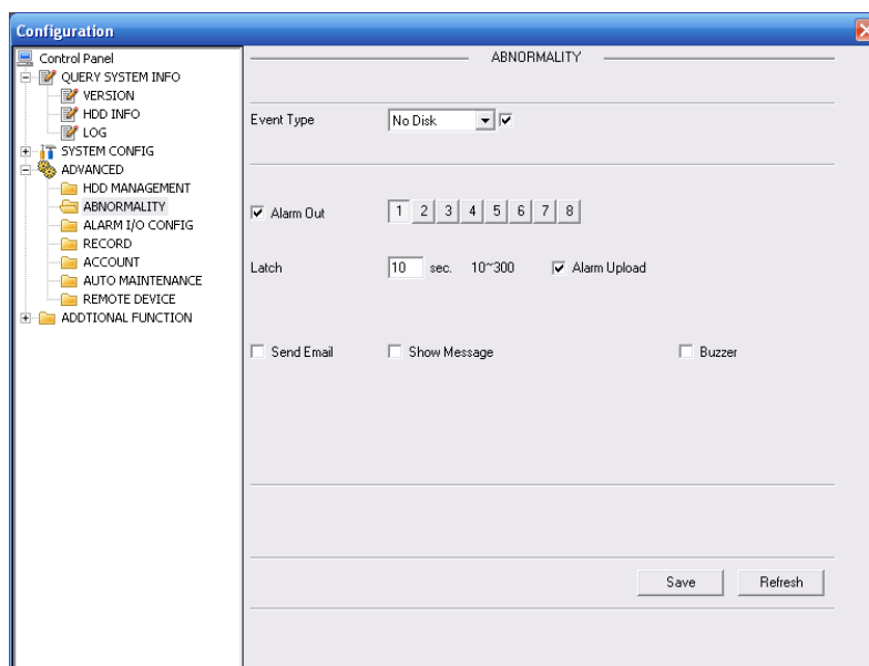
Figure 5-37 Abnormity -1
