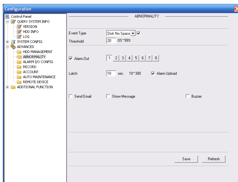
Figure 5-38 Abnormity -2
