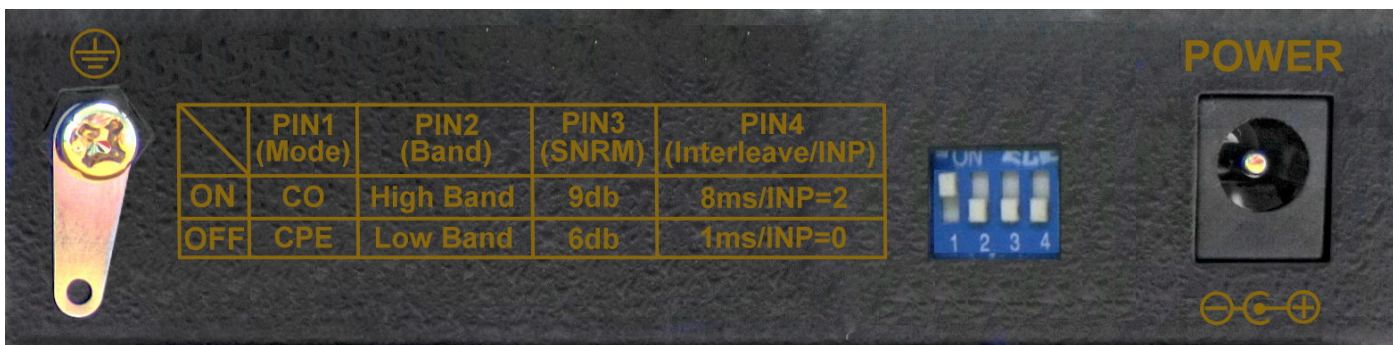
Figure 3.2 Rear Panel
