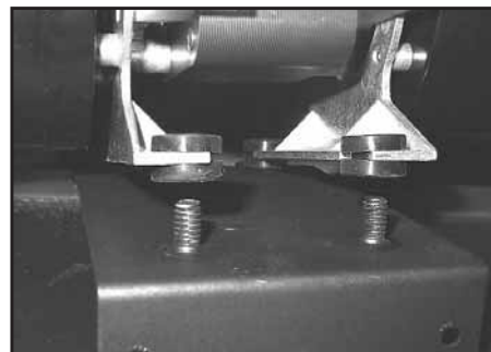
Figure 8.22 Install the new blower by slipping grommets over studs on the blower bracket. Reinstall the blower and bracket. Connect the wires. Install screws. Restore power to the appliance.
