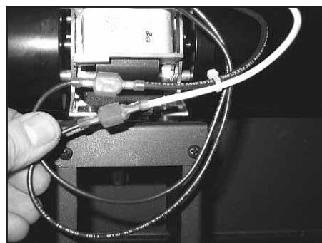
Figure 8.21 Disconnect wires to the blower motor. Remove the blower from the bracket.
