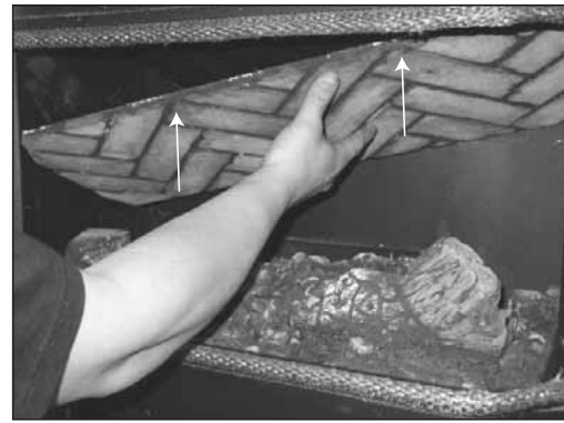
Figure 8.7 To install the baffle, slide it in at an angle and rotate upward parallel with the firebox. Place baffle up against the heat exchangers in top of firebox. Holding against heat exchangers, slide baffle towards front of appliance.
