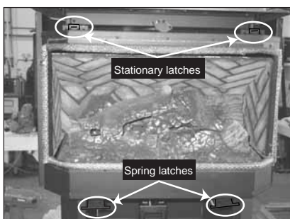
Figure 8.1 Open lower access panel. Pull out and unhook the two spring latches on the bottom of the appliance that secure the door.
