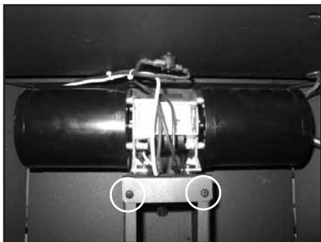
Figure 8.20 Disconnect power to the appliance. To access the blower, open the door located on the front of the pedestal. Remove the two screws holding the blower bracket in place.
