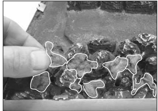
Figure 8.19 Place individual pieces of embers in front of and around the gas log where they can be seen. Space them so that gas can contact them on all sides. Avoid stacking the embers on top of each other.
