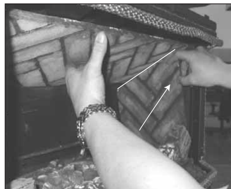
Figure 8.8 Keeping the baffle elevated with your free hand, put the right side brick into position. Rest the baffle on the right side brick.
