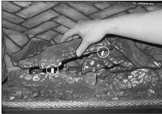
Figure 8.18 Install the left twig (#6) over the locator pins in the right rear log and the left front log.
