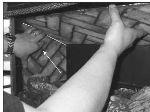
Figure 8.9 Still holding the baffle in place, install the left brick into position.
