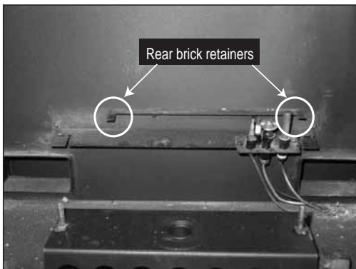
Figure 8.12 NOTE: For the Hudson Bay Free Standing the upper rear brick retainer is used.
