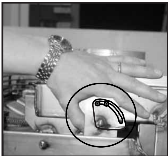
Figure 8.24 Open the right side panel to access the shutter adjustment.
