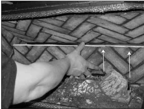
Figure 8.11 Install the rear brick. Slide it in at an angle and place over the rear brick retainer. Hand bend retaining tabs up to hold brick in place. Push baffle towards back of firebox.
