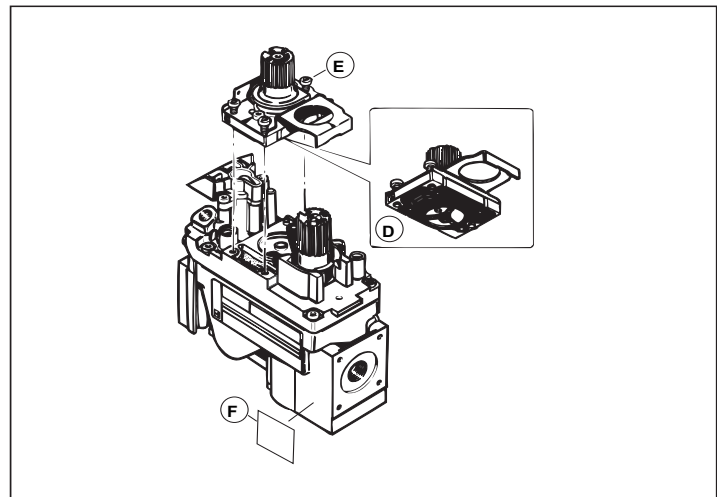
Figure 6.9 Ensure that the rubber gasket (D) is properly positioned and install the new HI/LO pressure regulator assembly to the valve using the new screws (E) supplied with the
