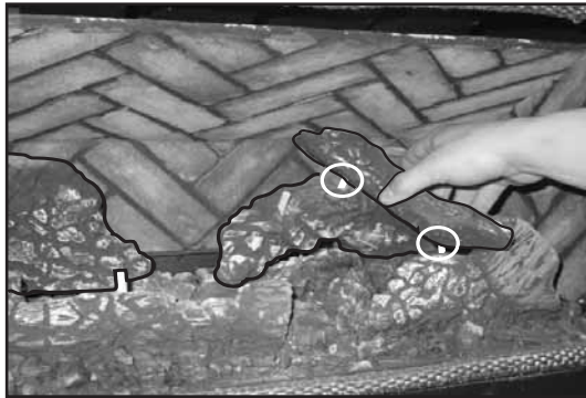
Figure 8.17 Install the right twig (#5) over the locator pins in the right rear log and the right front log.
