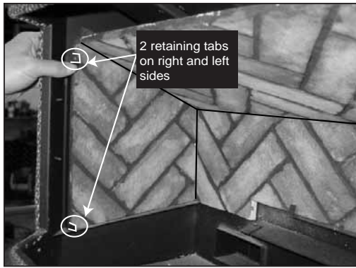
Figure 8.10 Bend retaining tabs on left and right sides inward to hold brick in place.
