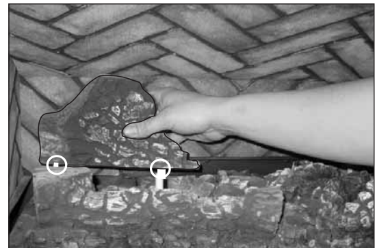
Figure 8.15 Install the left rear log (#3) over the locator pins in the burner pan.
