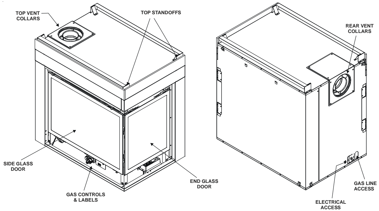
Figure 3. Diagram of the LCOR-HVB-IPI and RCOR-HVB-IPI
