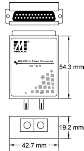
Fig. 1: RS-232 (DB25) Serial-Port Fiber Converter
