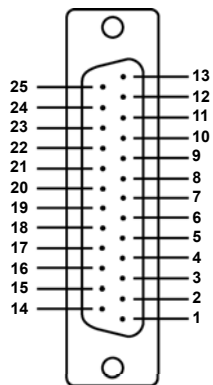
Fig. 3: DB25 Port Pinouts
