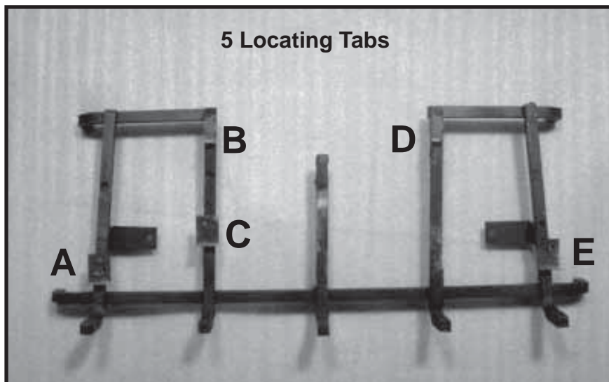
Grate Assembly
