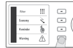
Spa warnings
