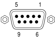
As viewed from the rear of the WJ-HD316A/WJ-HD309A
