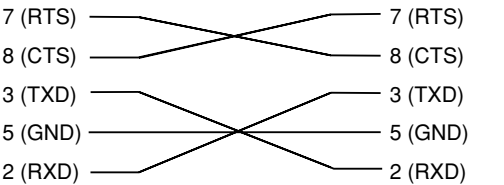
Cross cable connection example
