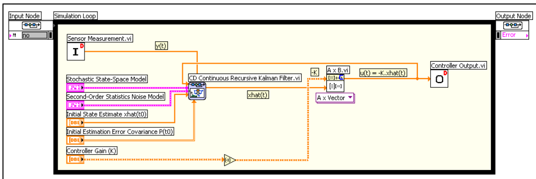
Figure 17-8. Implementing a Continuous Controller Model and a Continuous Kalman Filter on an RT Target
