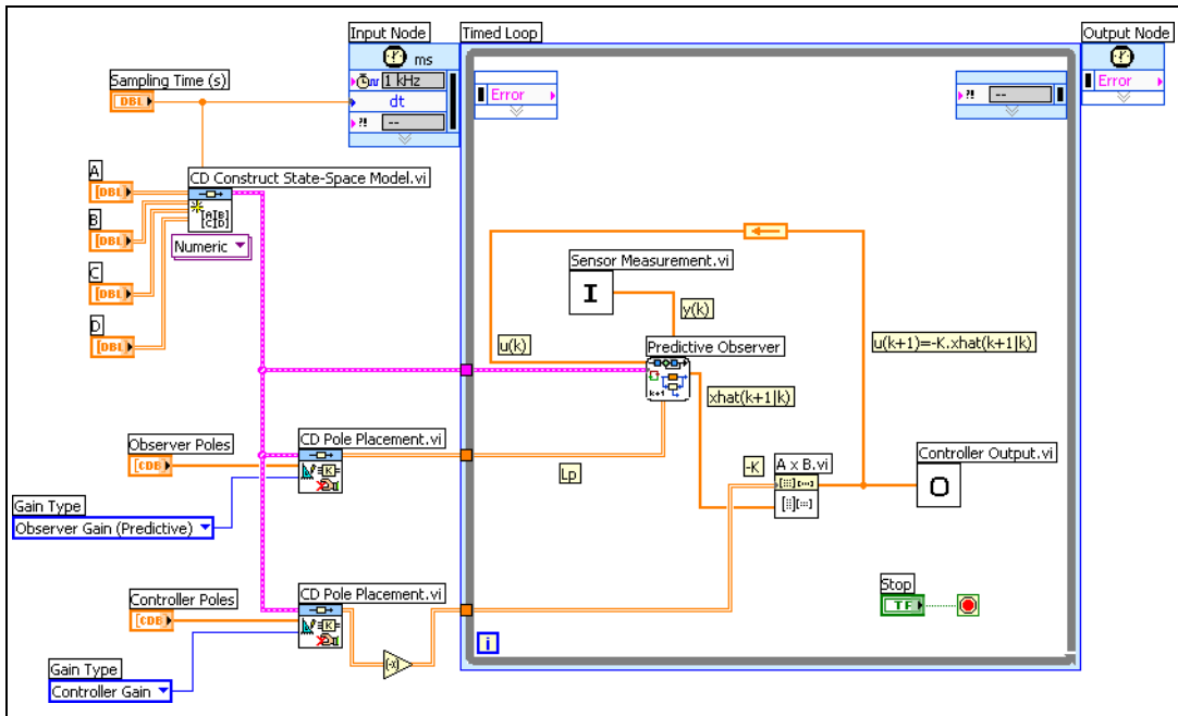
Figure 17-5. Implementing a Predictive Observer on an RT Target
