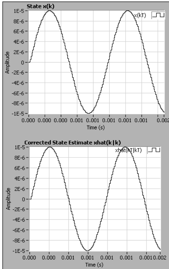
Figure 16-7. Actual Model States vs. Corrected State Estimates
