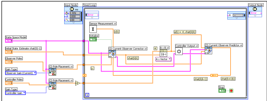
Figure 17-6. Implementing a Current Observer on an RT Target
