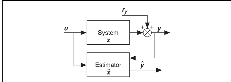
Figure 13-2. System Included State Estimator with Noise
