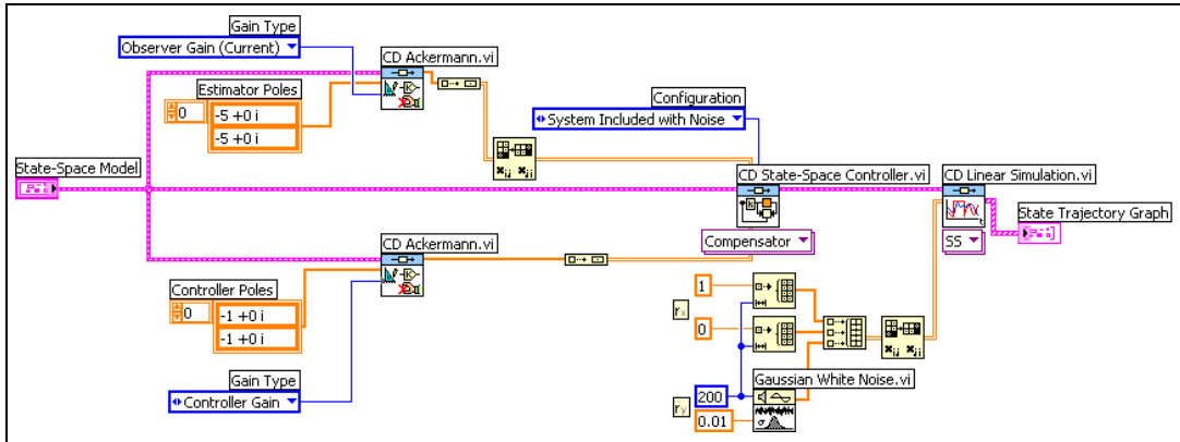
Figure 14-16. System Included State Compensator with Noise
