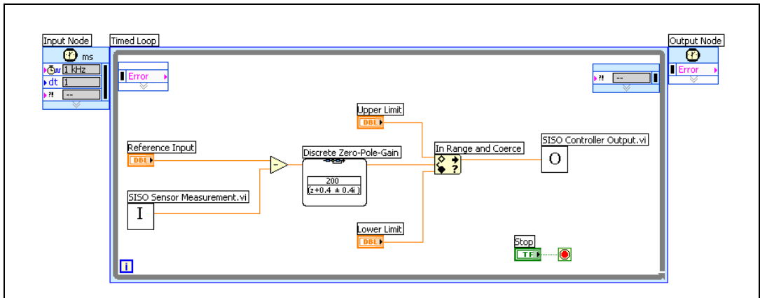
Figure 17-4. Implementing a Discrete Zero-Pole-Gain Controller on an RT Target
