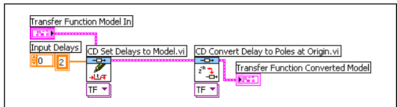
Figure 5-4. Adding Delay Information to a Discrete Transfer Function Model
