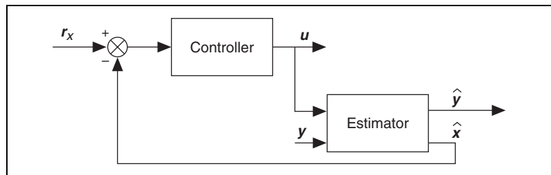
Figure 14-3. Standalone State Compensator with Estimator
