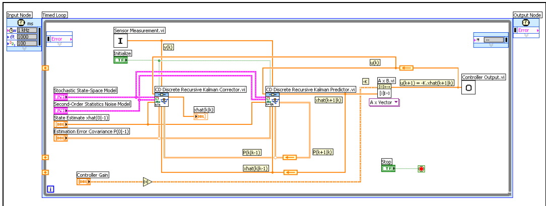
Figure 17-7. Implementing a Kalman Filter on an RT Target
