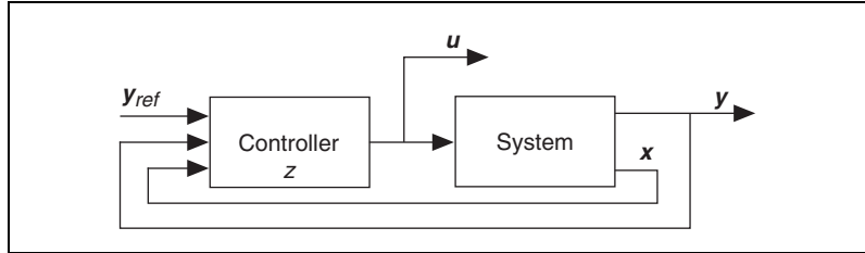
Figure 14-12. Standalone State Regulator with Integral Action, without Estimator
