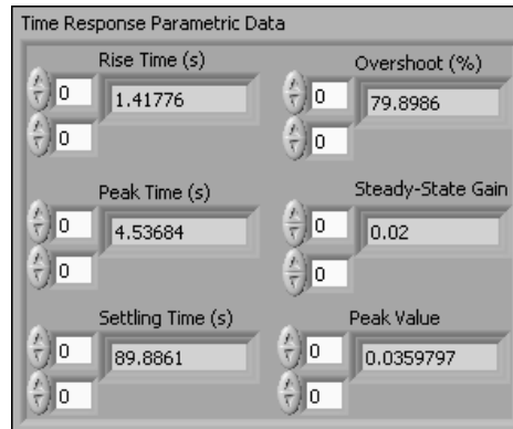
Figure 6-5. Parametric Data of the Spring-Mass Damper System
