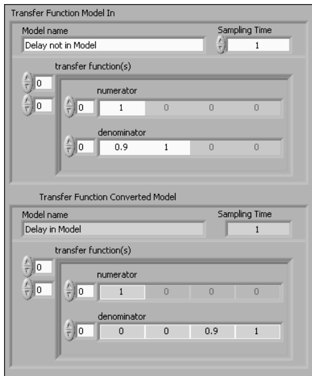
Figure 5-5. Additional Poles Accounting for the Input Delay
