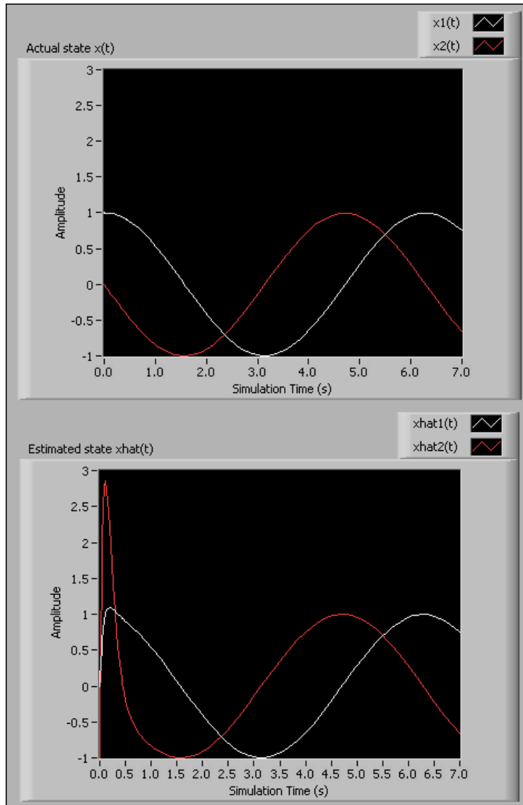
Figure 15-7. Actual Model States vs. Estimated Model States
