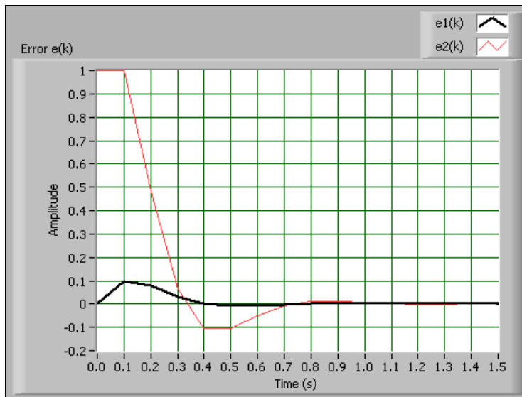
Figure 15-4. Estimation Error of a Predictive Observer
