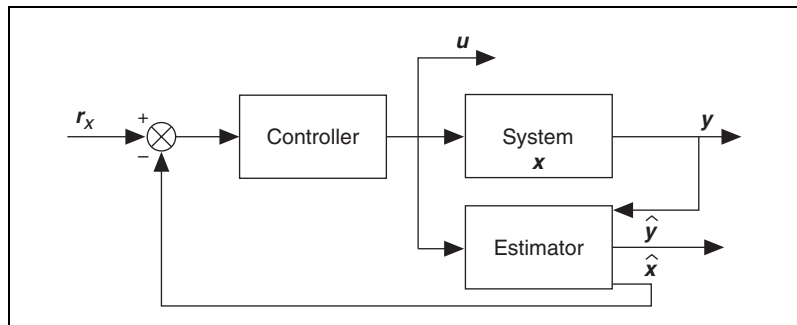
Figure 14-1. System Included State Compensator
