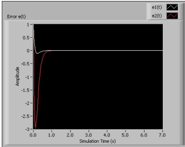
Figure 15-8. Estimation Error of a Continuous Observer
