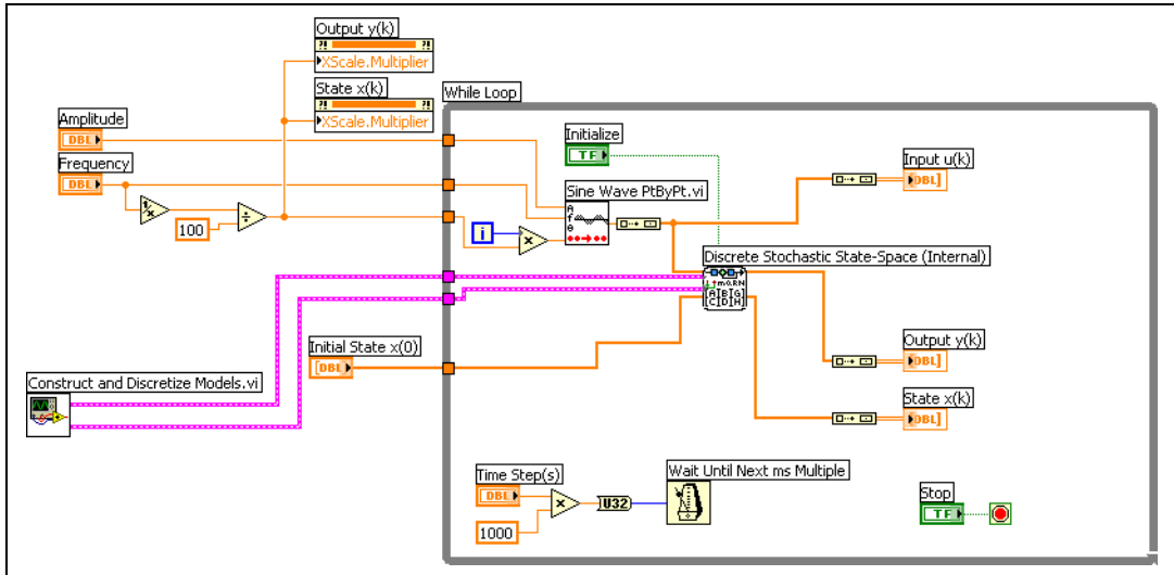
Figure 16-4. Simulating the Discrete Stochastic State-Space Model
