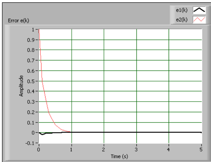
Figure 15-5. Estimation Error of a Current Observer
