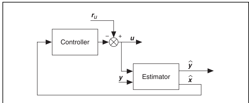
Figure 14-7. Standalone State Regulator with Estimator
