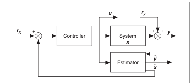
Figure 14-2. System Included State Compensator with Noise
