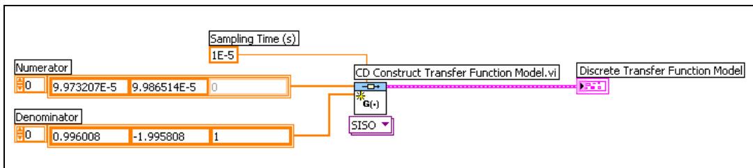
Figure 2-4. Using Coefficients to Create a Discrete Transfer Function Model
