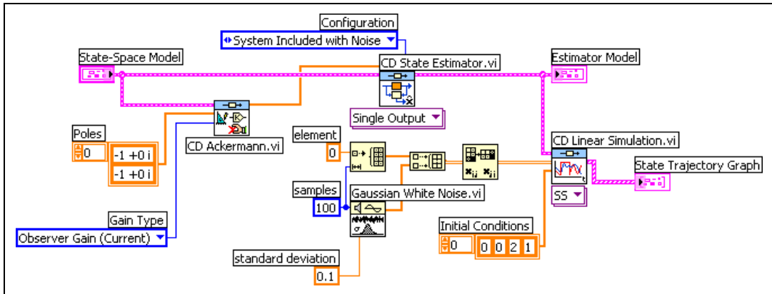
Figure 13-6. System Included State Estimator with Noise
