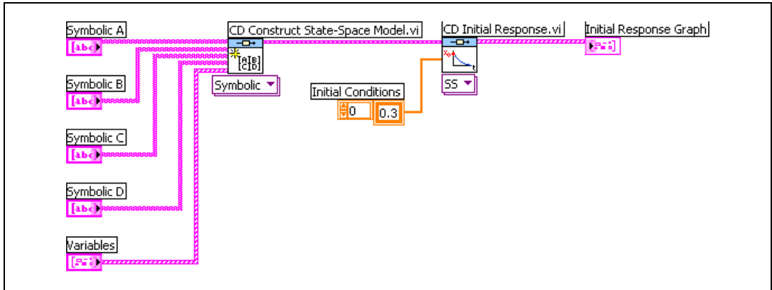
Figure 6-8. Initial Response Block Diagram of the Spring-Mass Damper System
