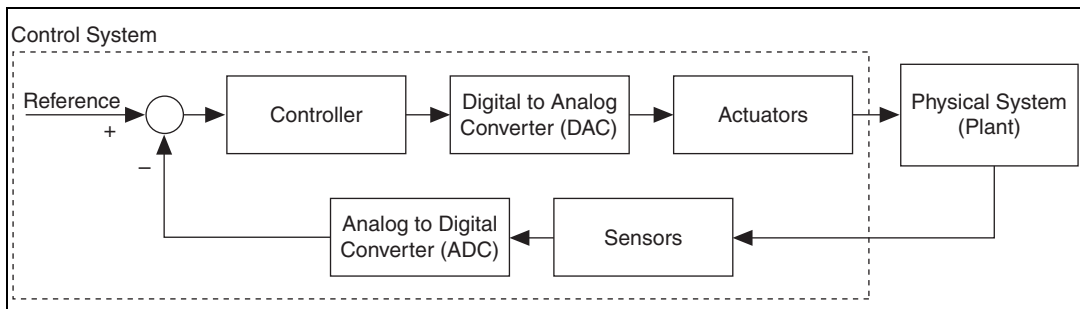
Figure 17-1. Closed-Loop Dynamic System
