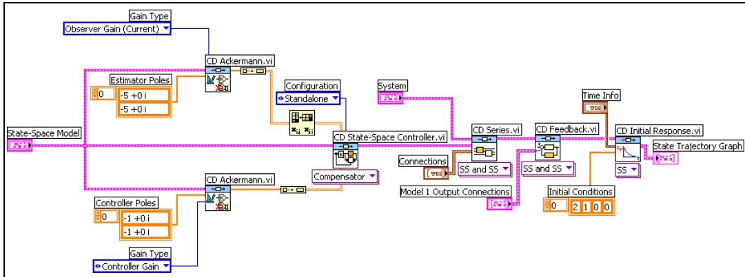
Figure 14-18. Standalone State Compensator with Estimator
