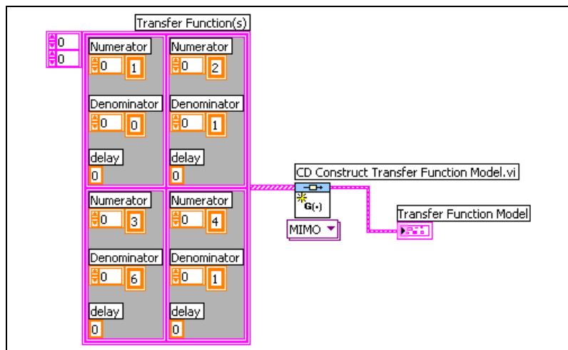
Figure 2-7. Creating a MIMO Transfer Function Model
