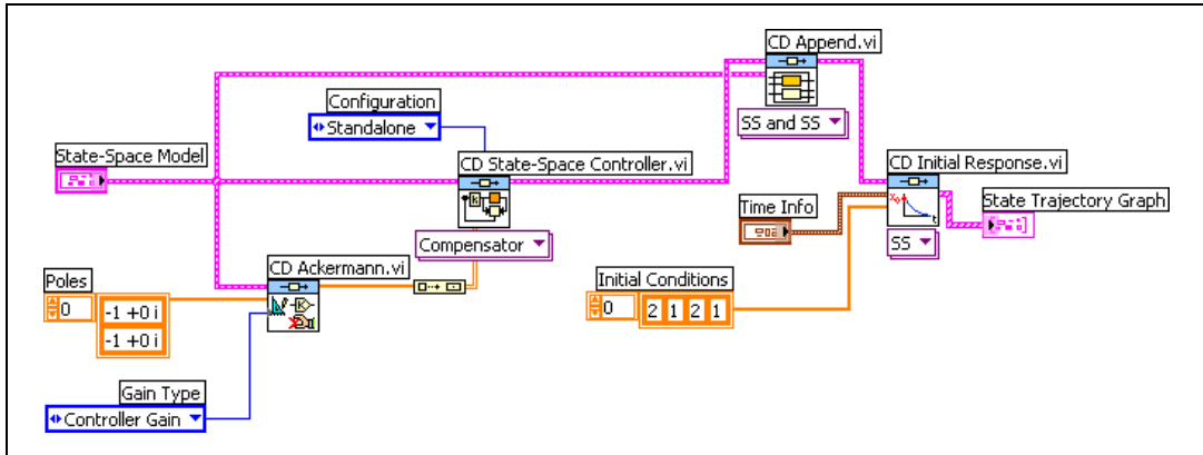
Figure 14-20. Standalone Compensator without Estimator
