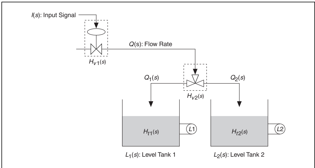
Figure 4-3. Dividing the Flow of Water between Two Tanks
