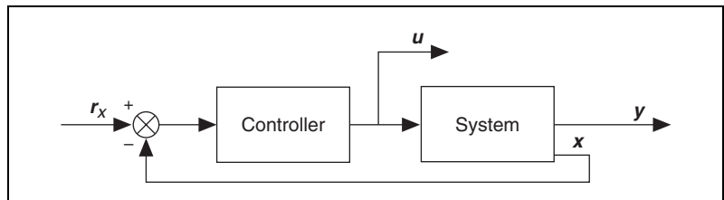
Figure 14-4. Standalone State Compensator without Estimator
