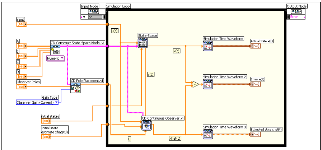
Figure 15-6. Implementing a Continuous Observer for a State-Space Model
