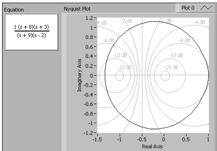
Figure 7-2. Nyquist Plot of One Unstable Pole
