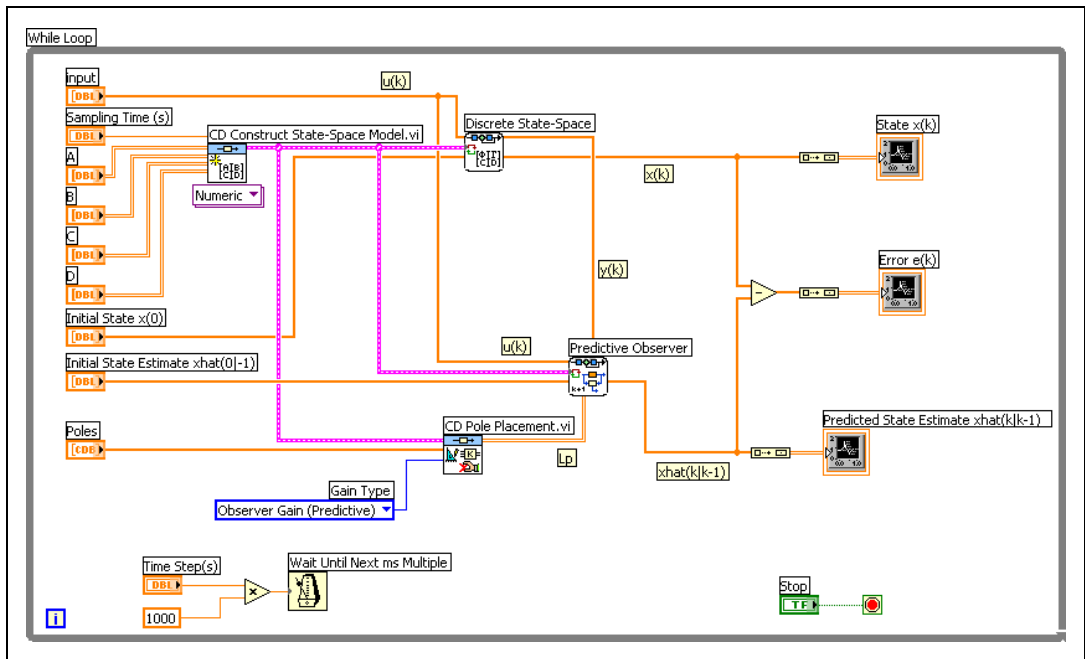
Figure 15-2. Implementing a Predictive Observer for the State-Space Model
