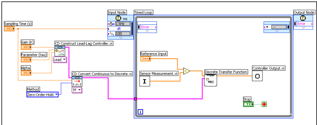
Figure 17-2. Implementing a Discrete Transfer Function Controller on an RT Target
