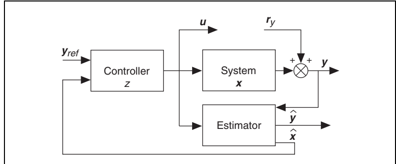
Figure 14-10. System Included State Regulator with Integral Action, with Noise
