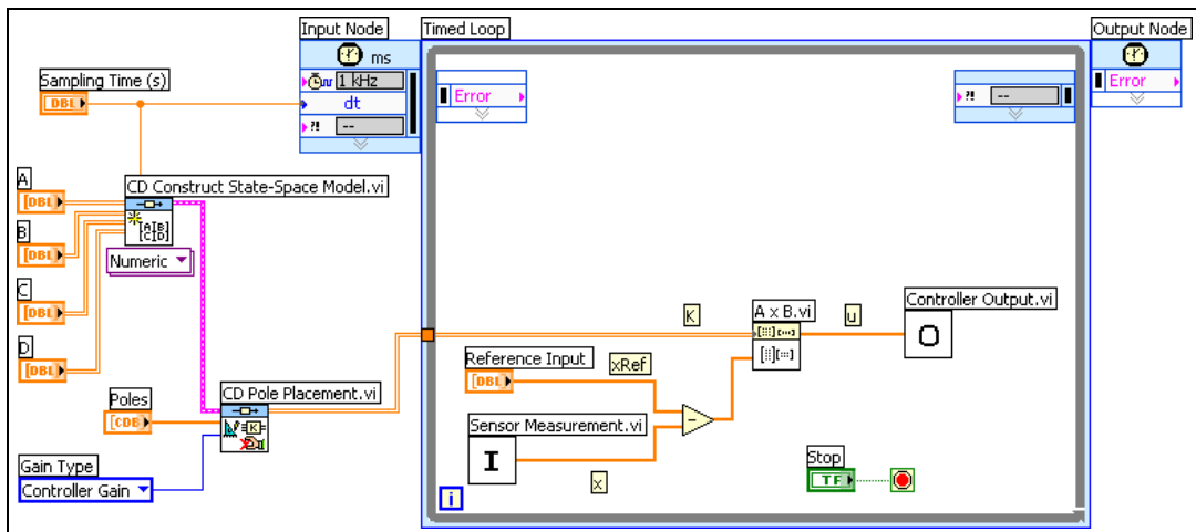
Figure 17-3. Implementing a State Compensator on an RT Target
