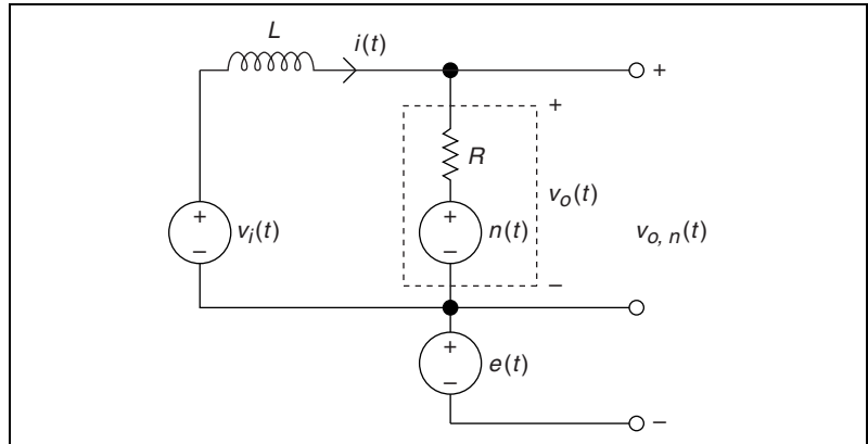
Figure 16-1. Noisy RL Circuit
