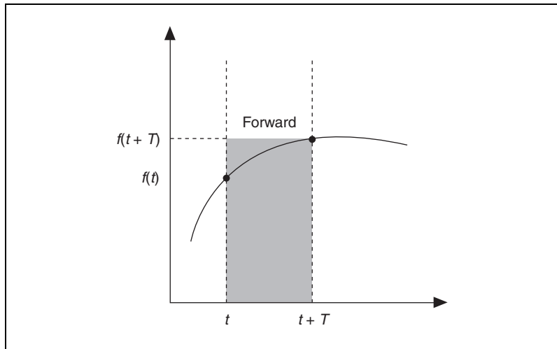
Figure 3-2. Forward Rectangular Method
