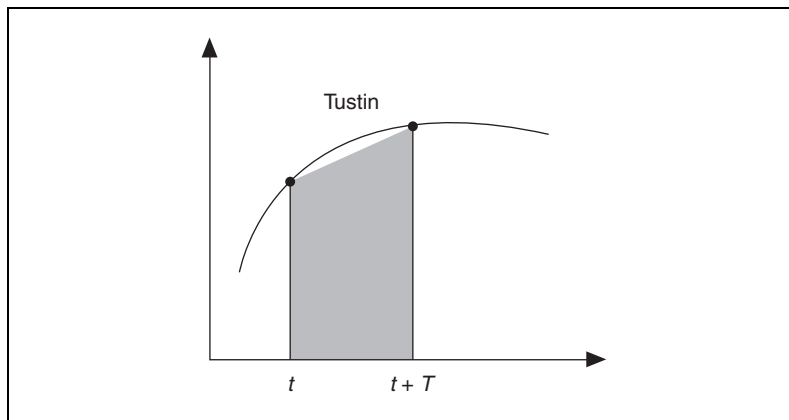
Figure 3-4. Tustin's Method
