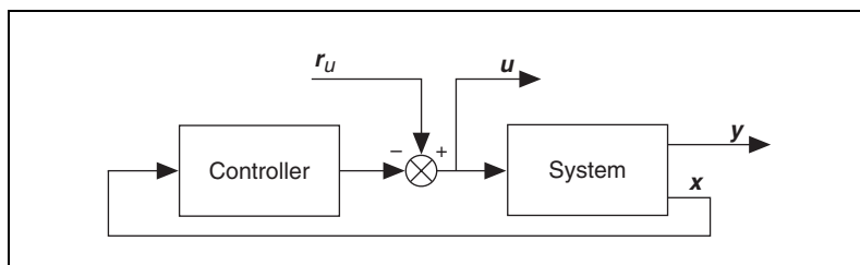
Figure 14-8. Standalone State Regulator without Estimator
