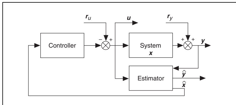
Figure 14-6. System Included State Regulator with Noise
