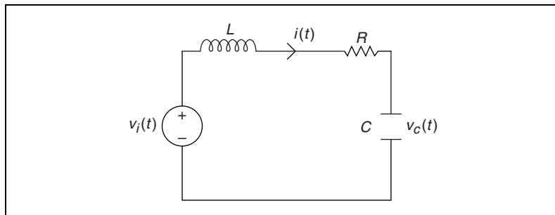
Figure 2-2. RLC Circuit
