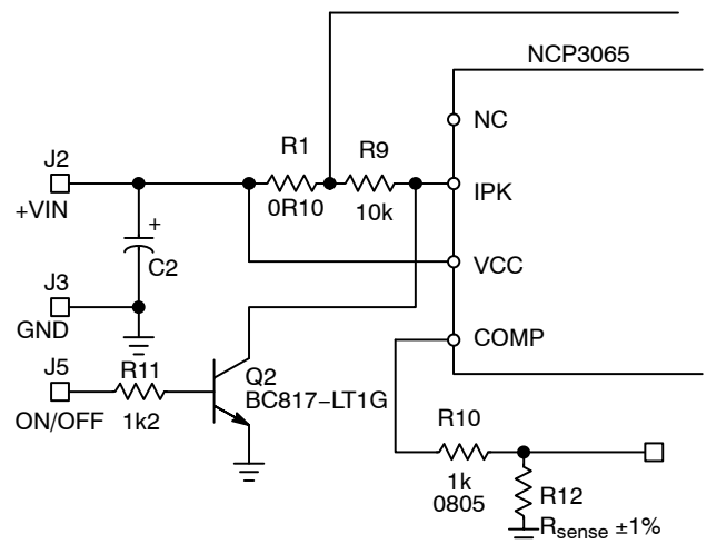
Figure 5. NCP3065 Dimming Solution B
