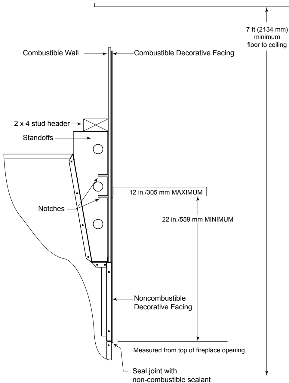
→ Figure 12.11 Clearances to Mantels or other Combustibles above Fireplace
