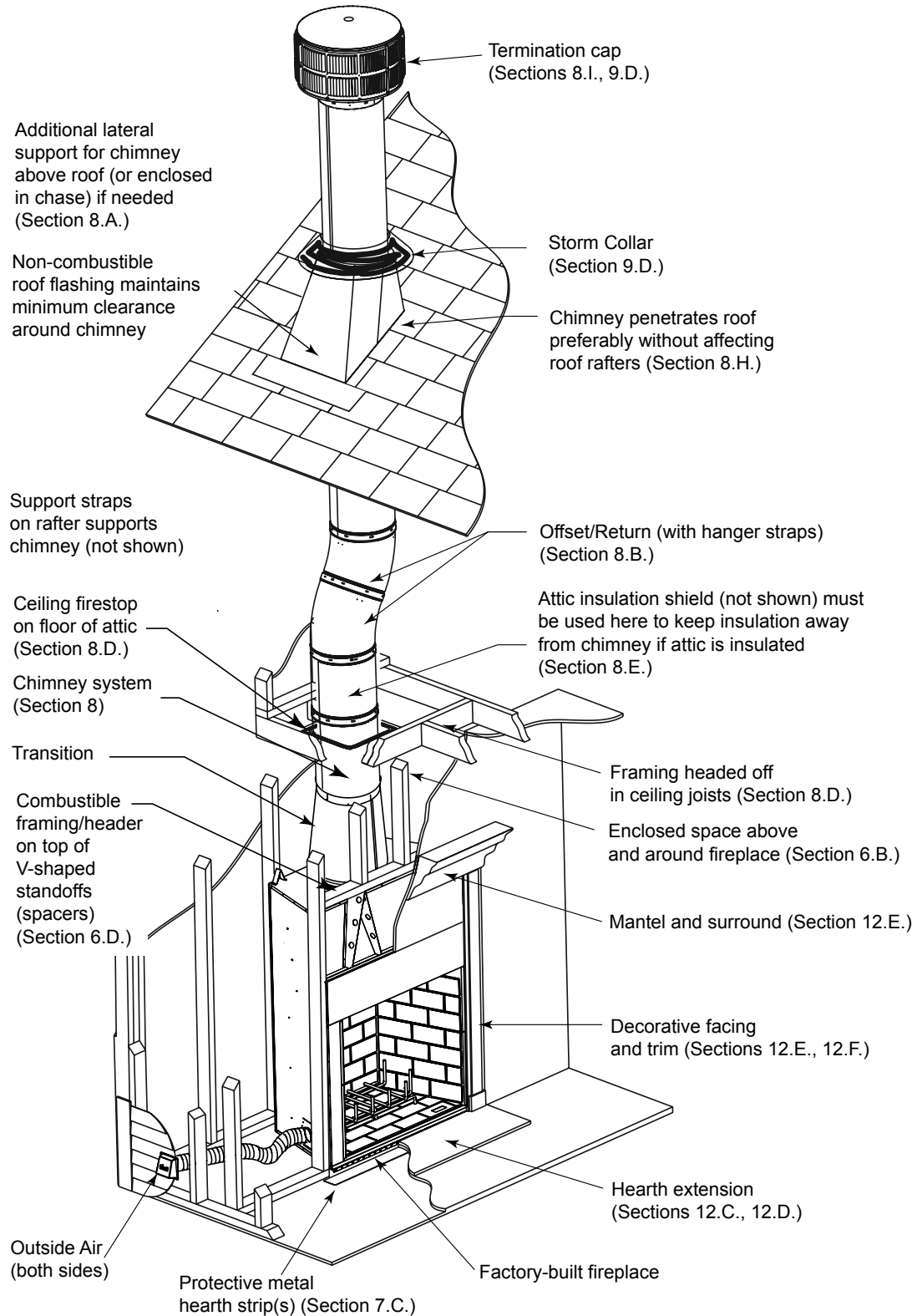
Figure 5.1 Typical Fireplace System
