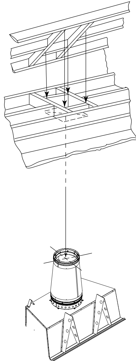
Figure 8.9 Ceiling/Attic Construction
